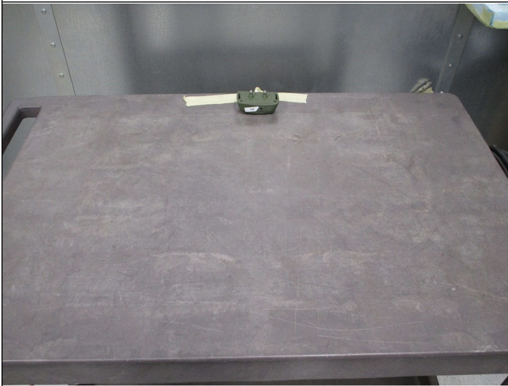
Test Setup for RF Conducted Emissions (AC Mains)
