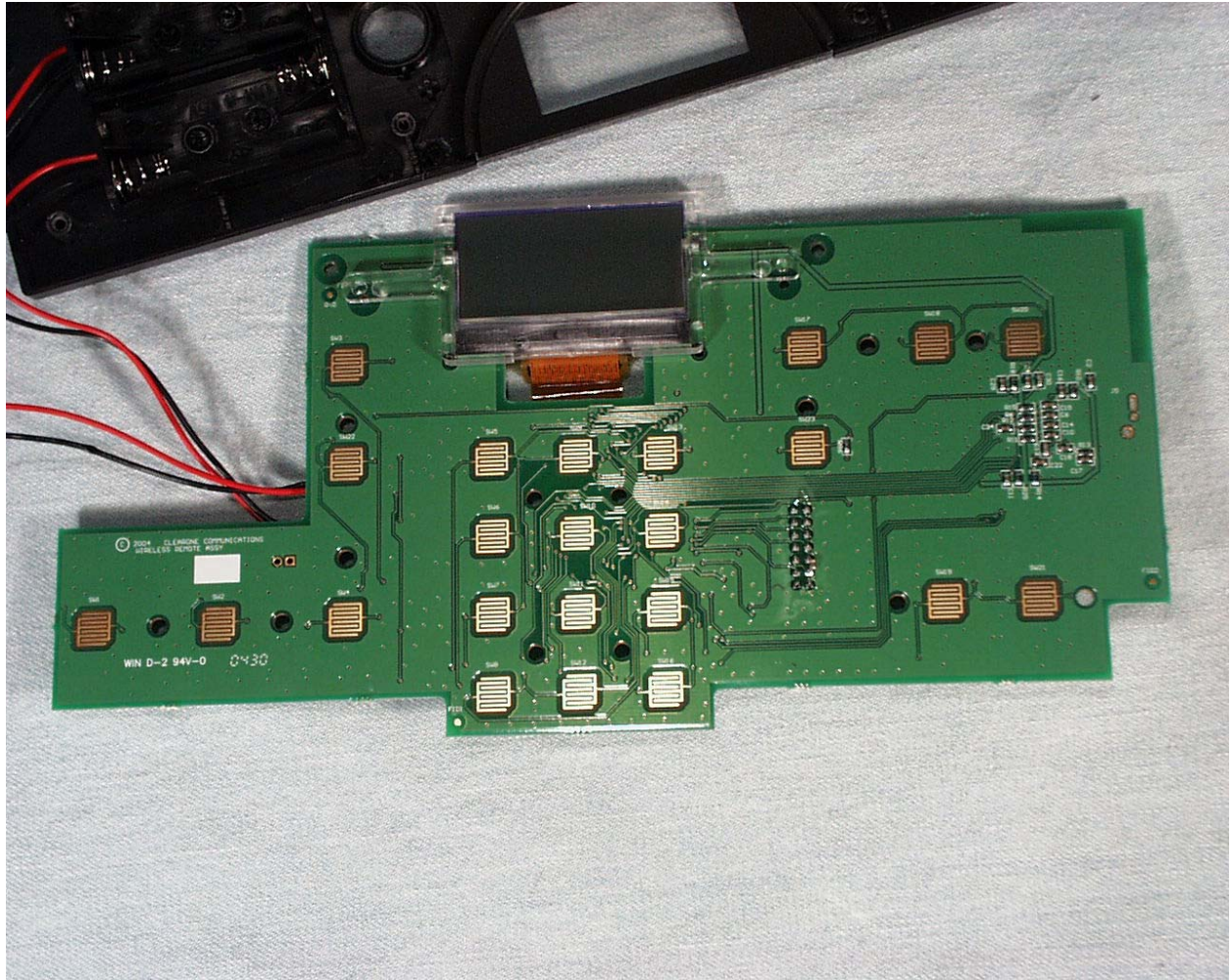
Trace Side of the EUT PC Board
