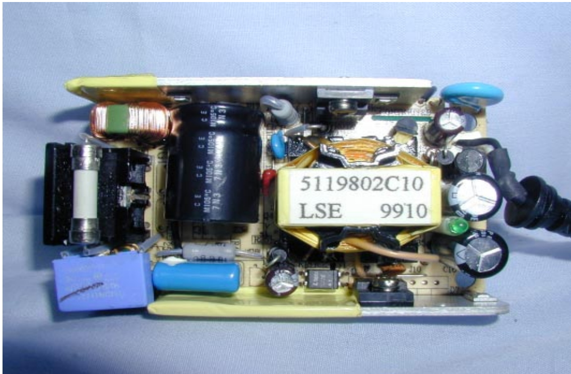
Main Board Component Side View of Adaptor
