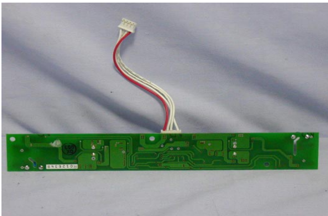
Main Board Solder Side View of Inverter
