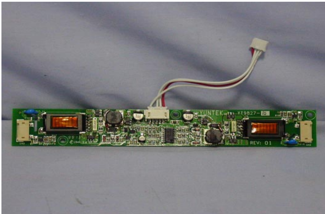
Main Board Component Side View of Inverter
