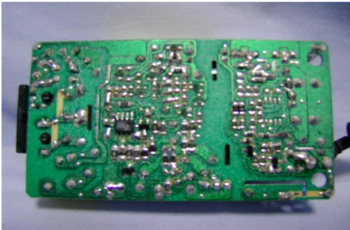
Main Board Solder Side View of Adaptor
