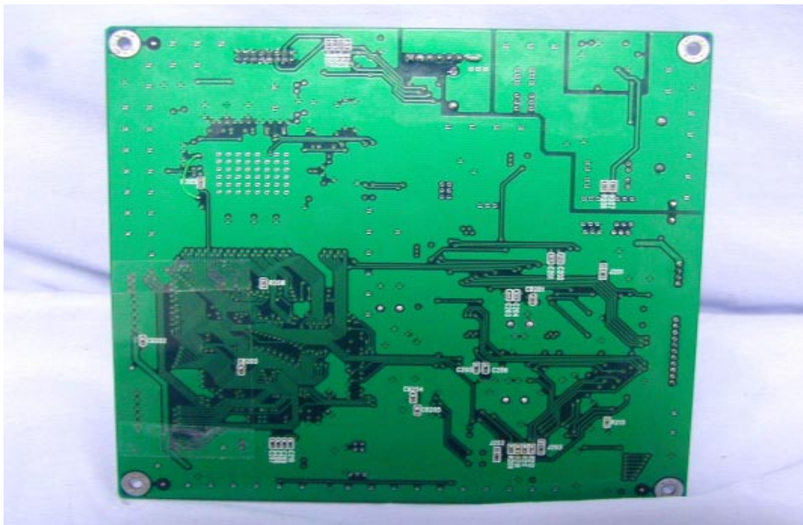
Main Board Solder Side View of EUT
