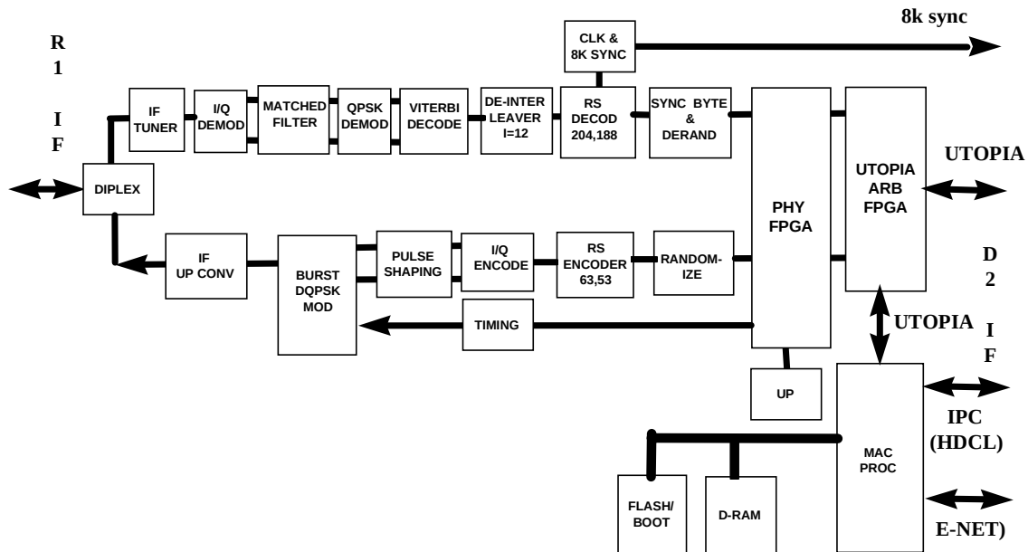
Figure 1.11 TDMA CPE Modem Block Diagram
