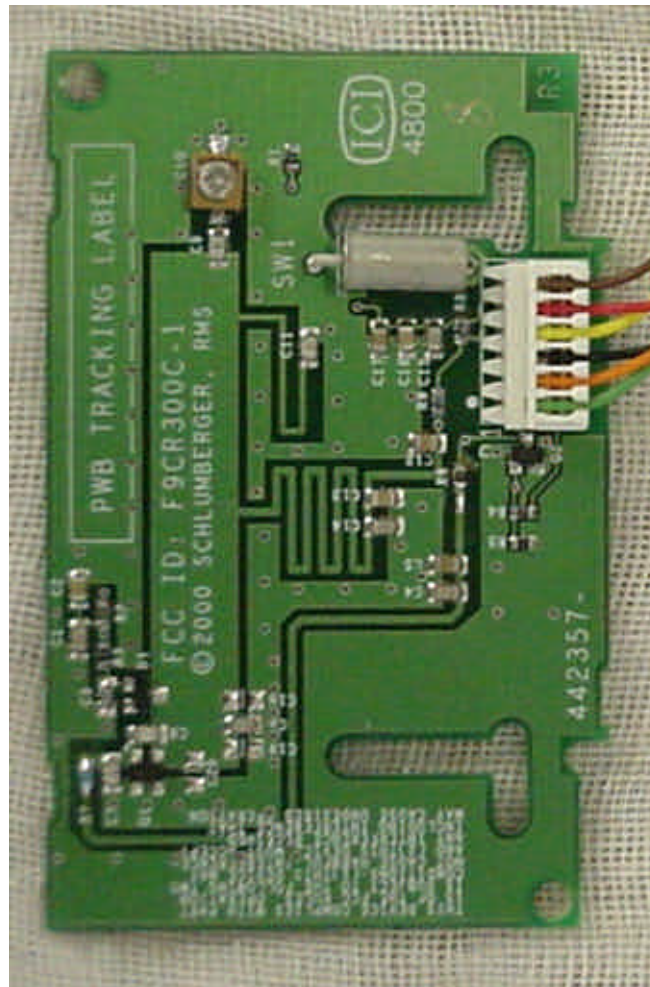
Photo 10. EUT, Top View of Transmitter Board
