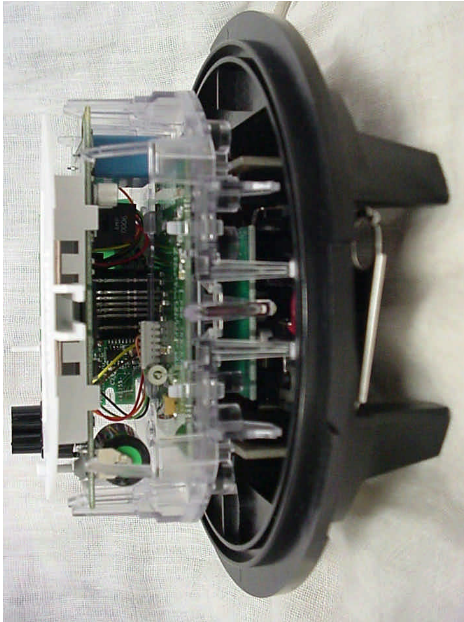
Photo 4. EUT, Side View with Plastic Cover Removed
