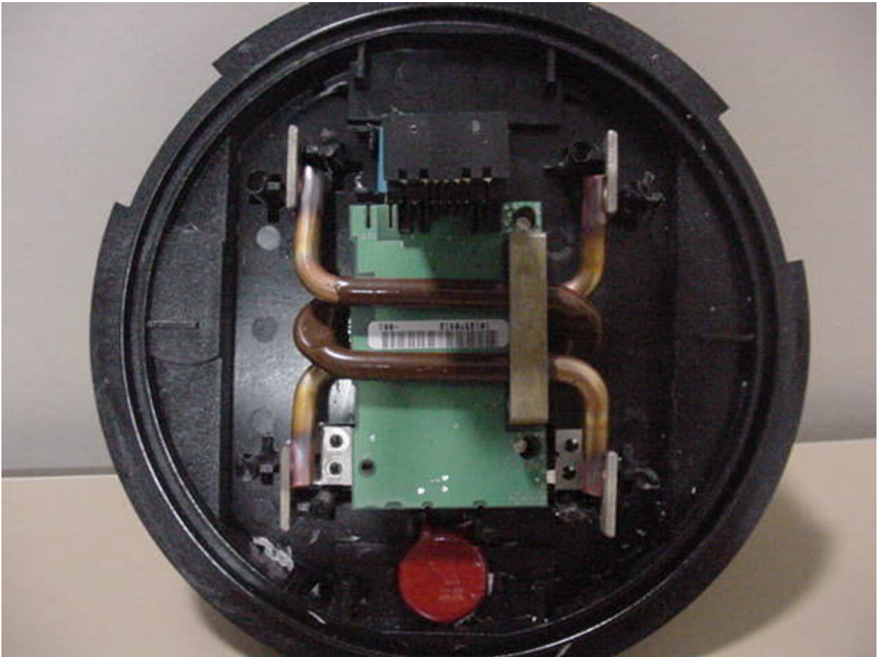
Figure B4: Meter Module – RF Board Removed Exposing Metrology Board
