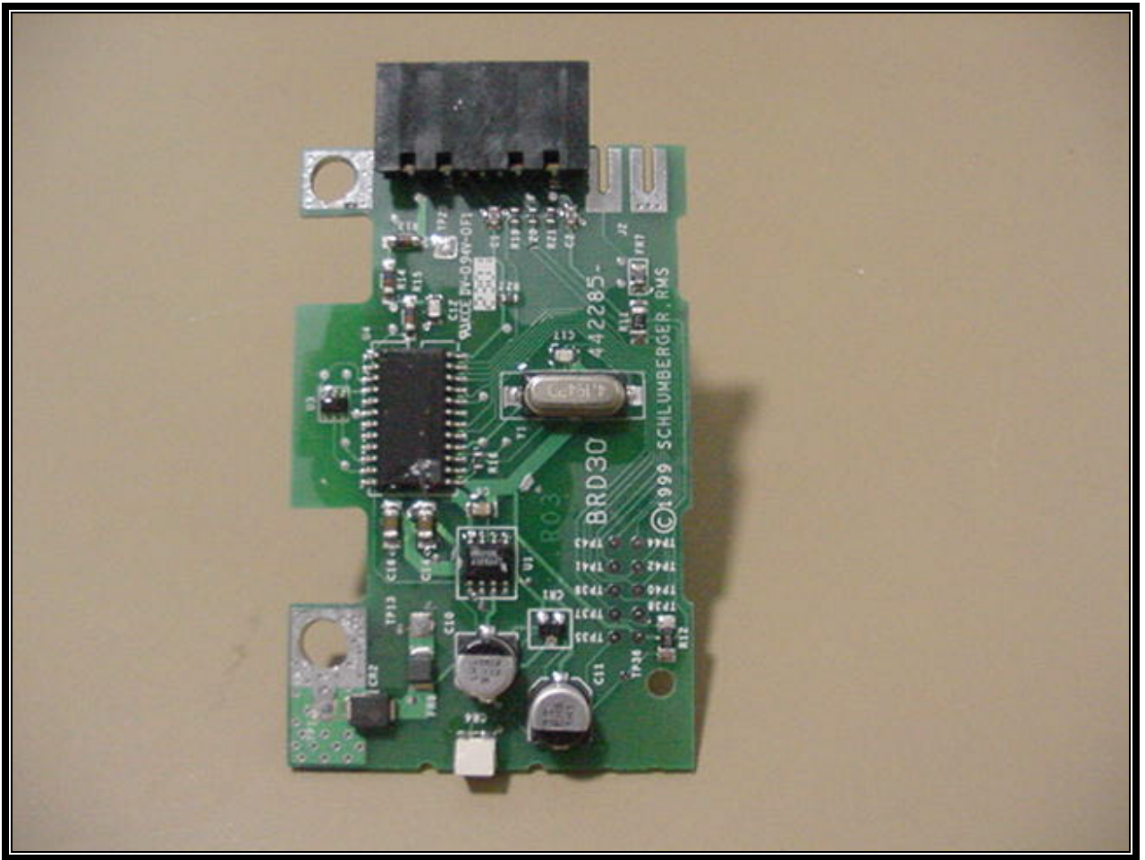
Figure B9: Metrology Board Top View
