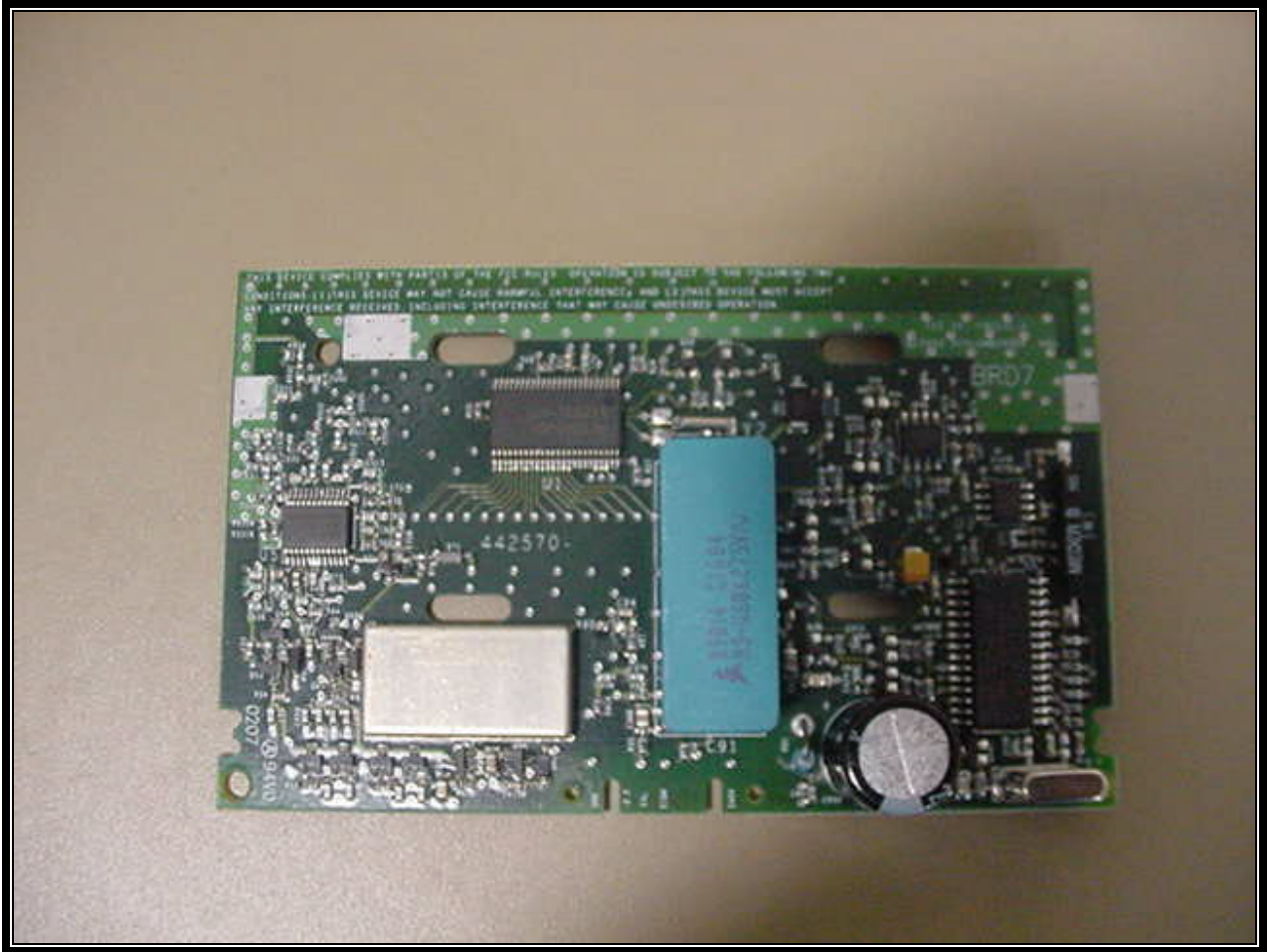
Figure B6: RF Board With Shield Top View
