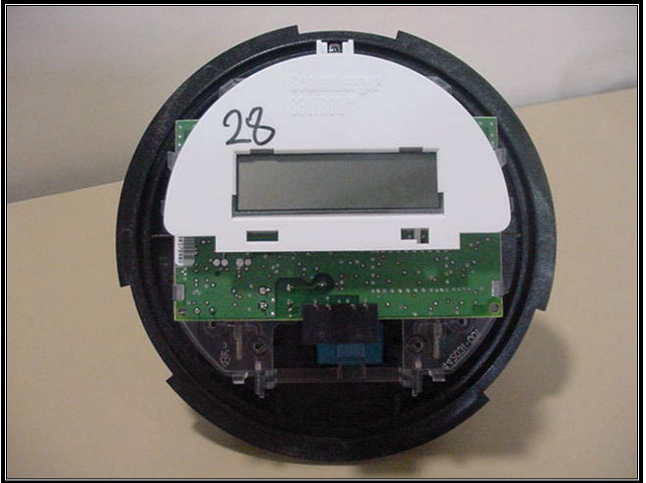
Figure B3: Meter Module with Cover Removed Exposing RF Board
