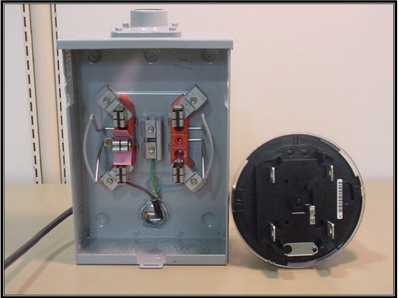
Figure C1: Meter Base and Rear View of Meter
