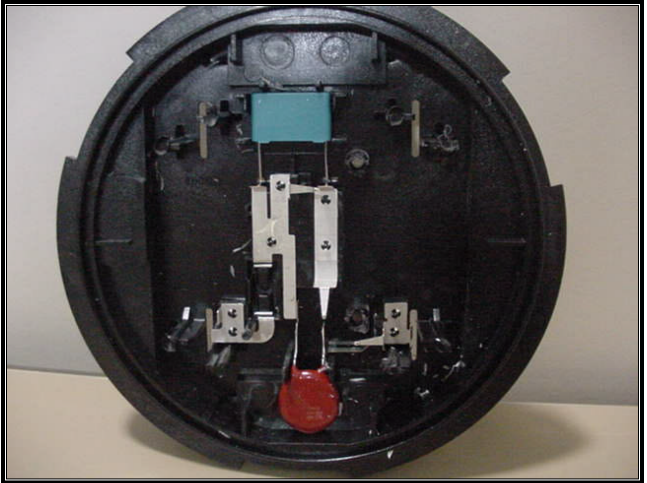
Figure B5: Meter Module All Boards Removed
