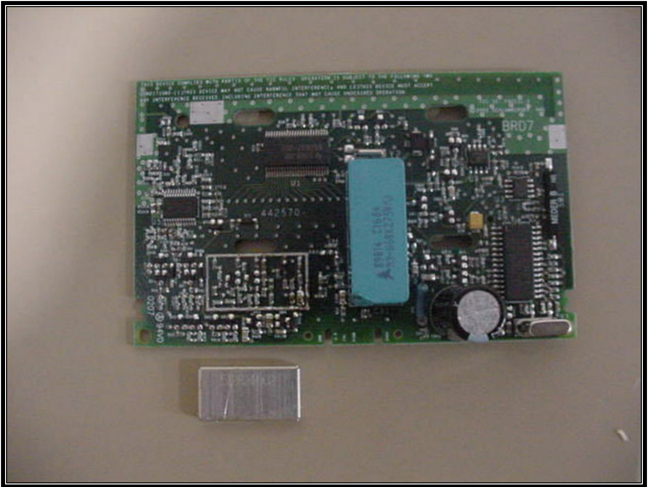
Figure B7: RF Board No Shield Top View
