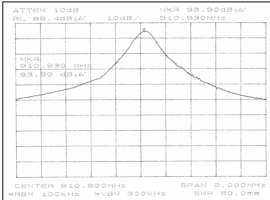
Figure 6.4.2-1: Peak Output Power – Low Channel
