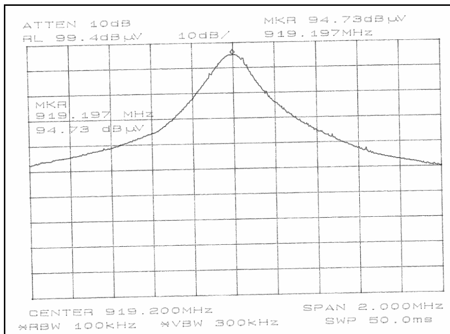
Figure 6.4.2-2: Peak Output Power – Low Channel
