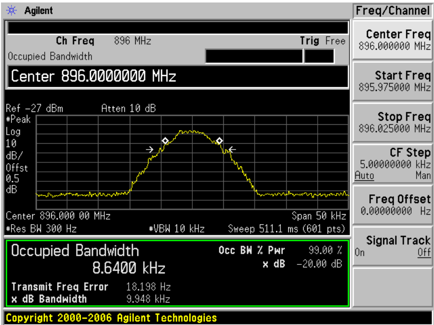
Output (C4FM P25)
