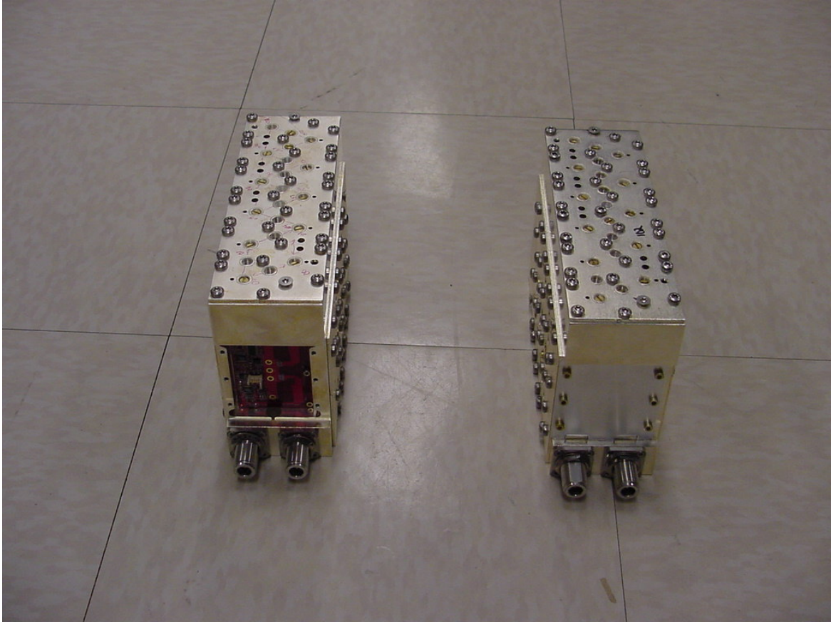
FlexWave™ URH Duplexer - PCS Bottom View
