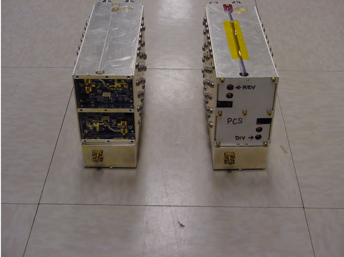
FlexWave™ URH Duplexer - PCS Front View
