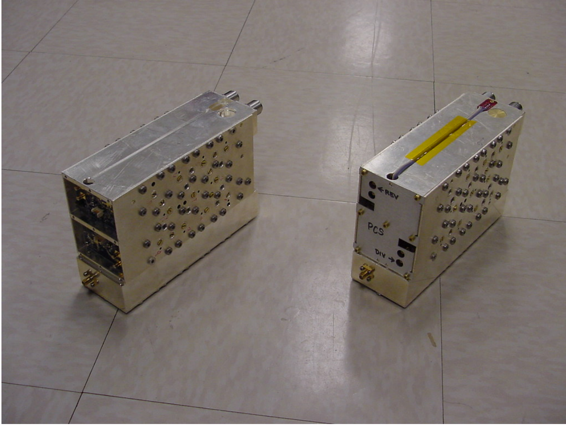
FlexWave™ URH Duplexer - PCS Right View
