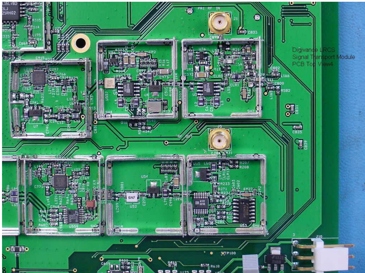
Digivance LRCS Signal Transport Module PCB Top View3
