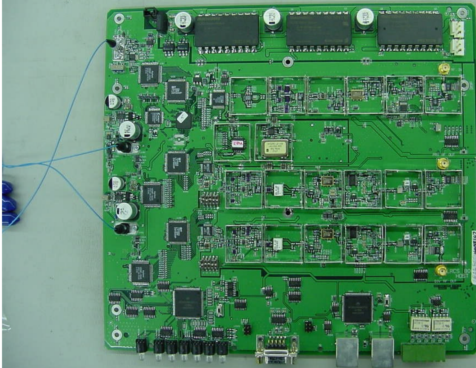
Digivance LRCS 800 MHz Host Control Board - Top View
