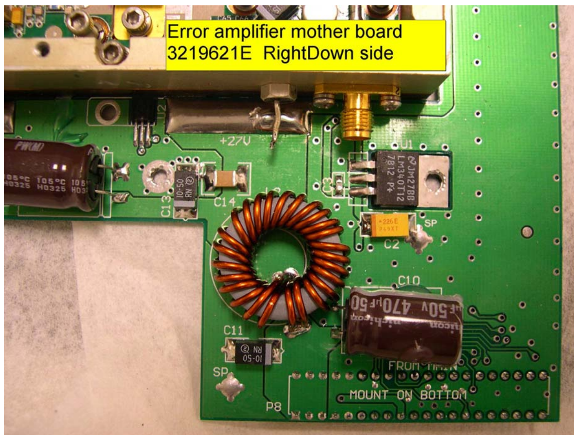
1900 MHz Linear Power Amplifier Error amplifier mother board 3219621E RightDown
