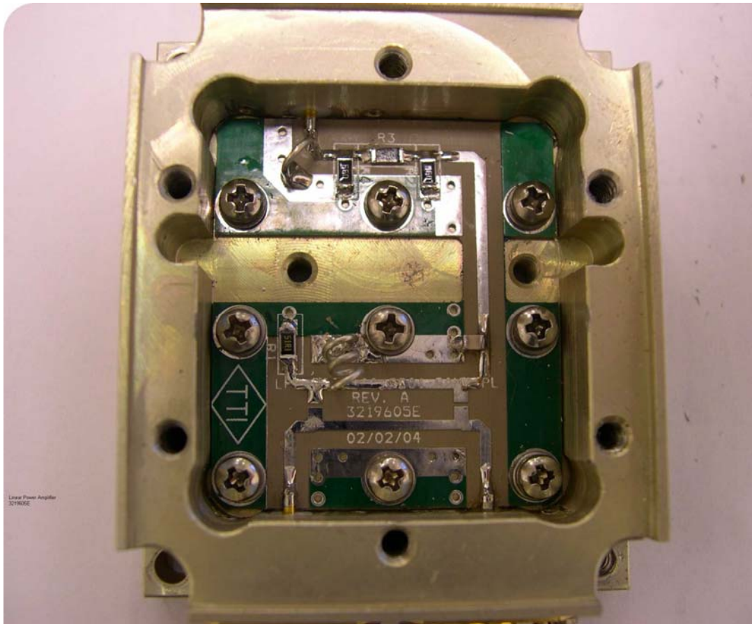
1900 MHz Linear Power Amplifier 3219605e
