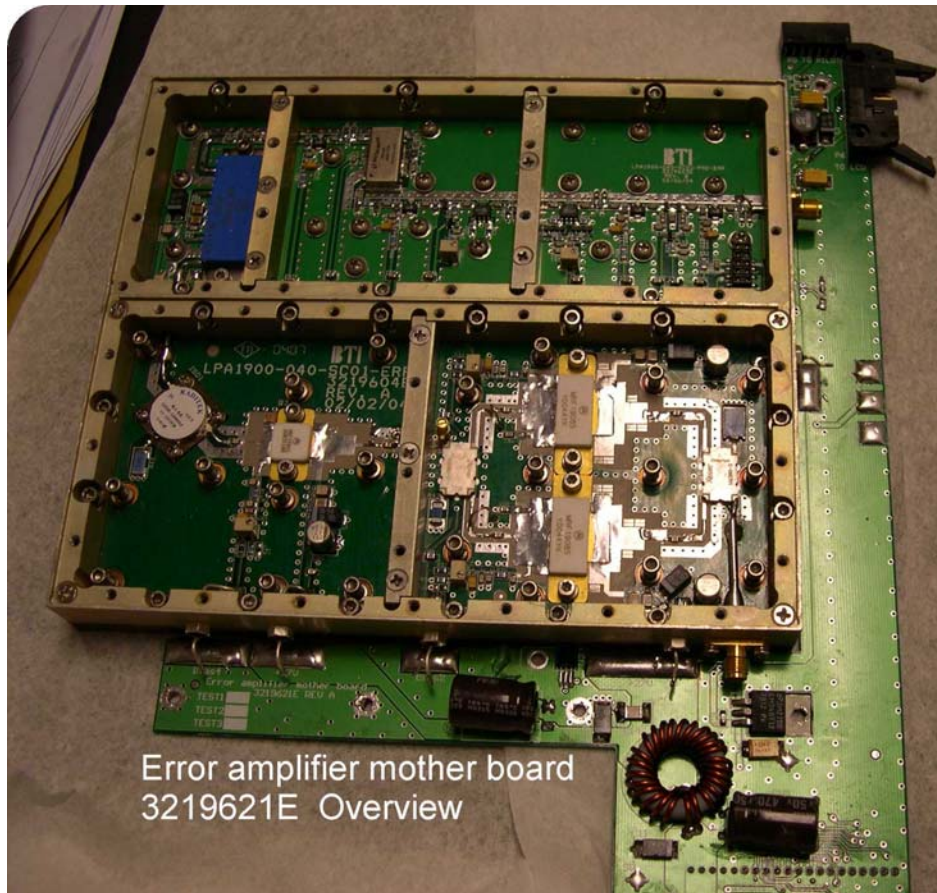
1900 MHz Linear Power Amplifier Error amplifier mother board 3219621E Overview
