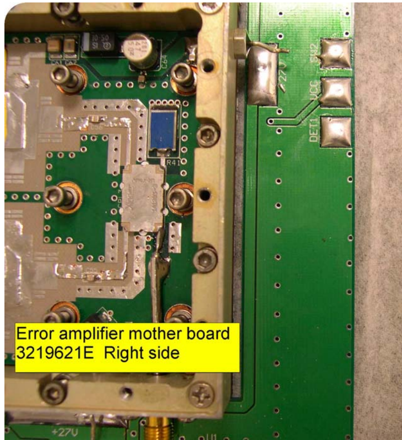
1900 MHz Linear Power Amplifier Error amplifier mother board 3219621E Right
