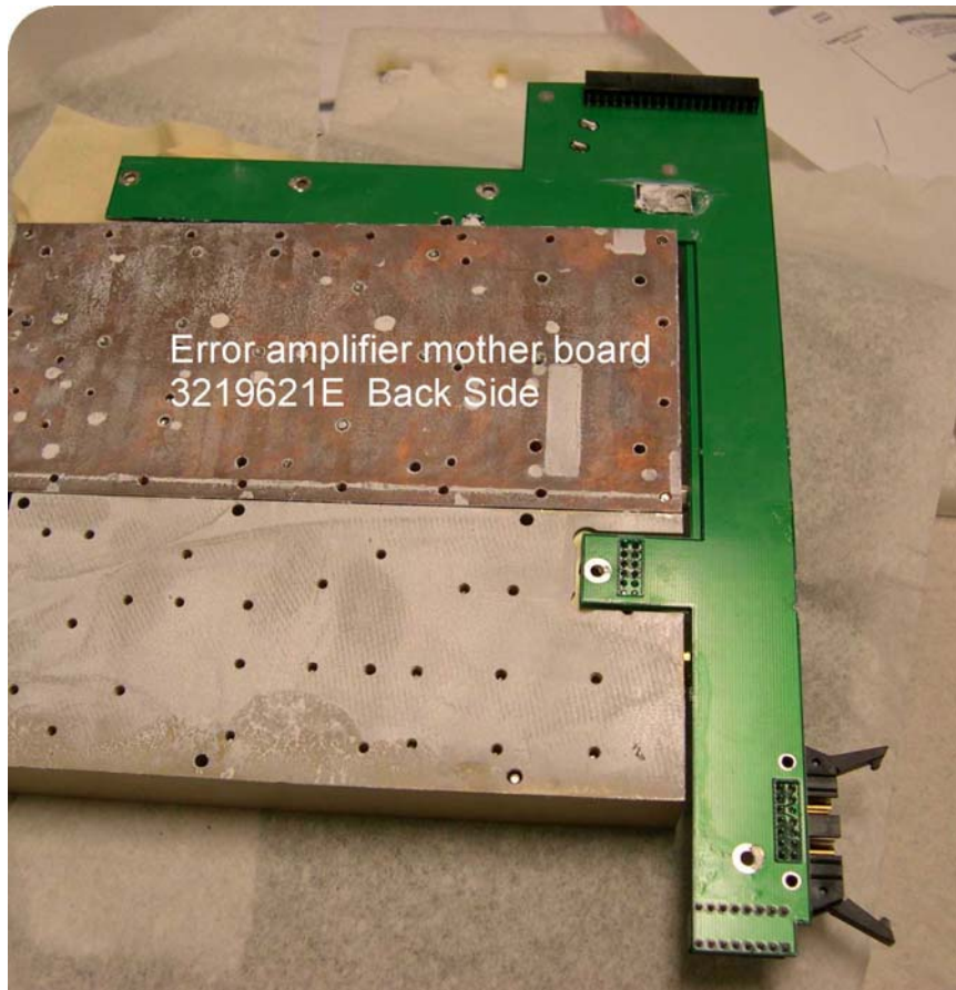
1900 MHz Linear Power Amplifier Error amplifier mother board 3219621E Back
