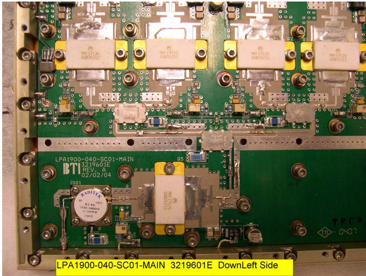
1900 MHz Linear Power Amplifier LPA1900-040-SC01-MAIN 3219601E DownLeft
