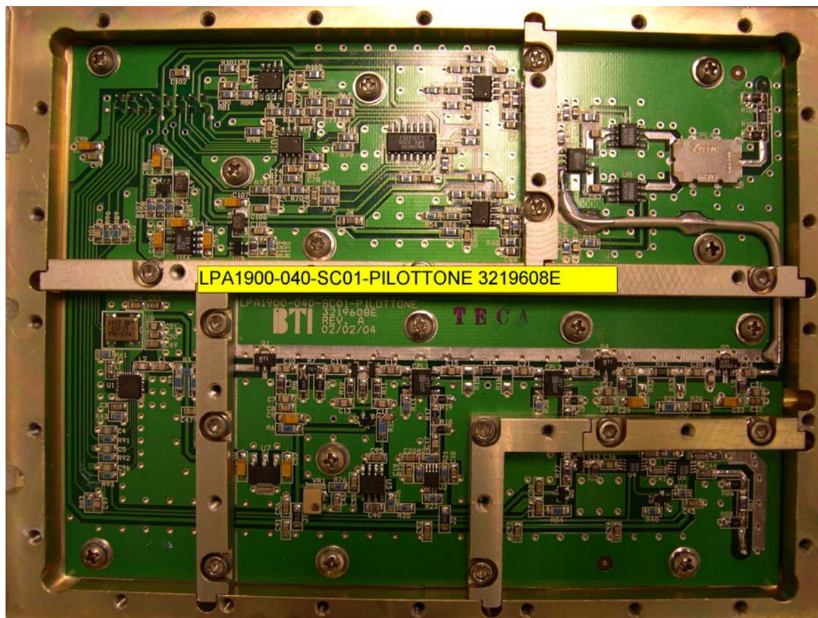
1900 MHz Linear Power Amplifier LPA1900-040-SC01-PILOTTONE 3219608E
