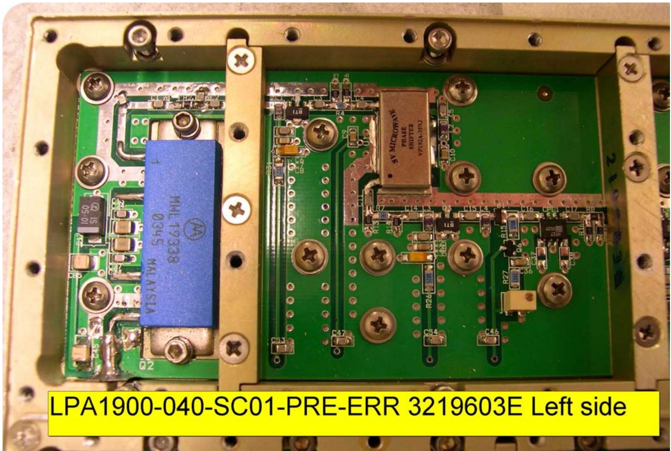
1900 MHz Linear Power Amplifier LPA1900-040-SC01-PRE-ERR 3219603E Left
