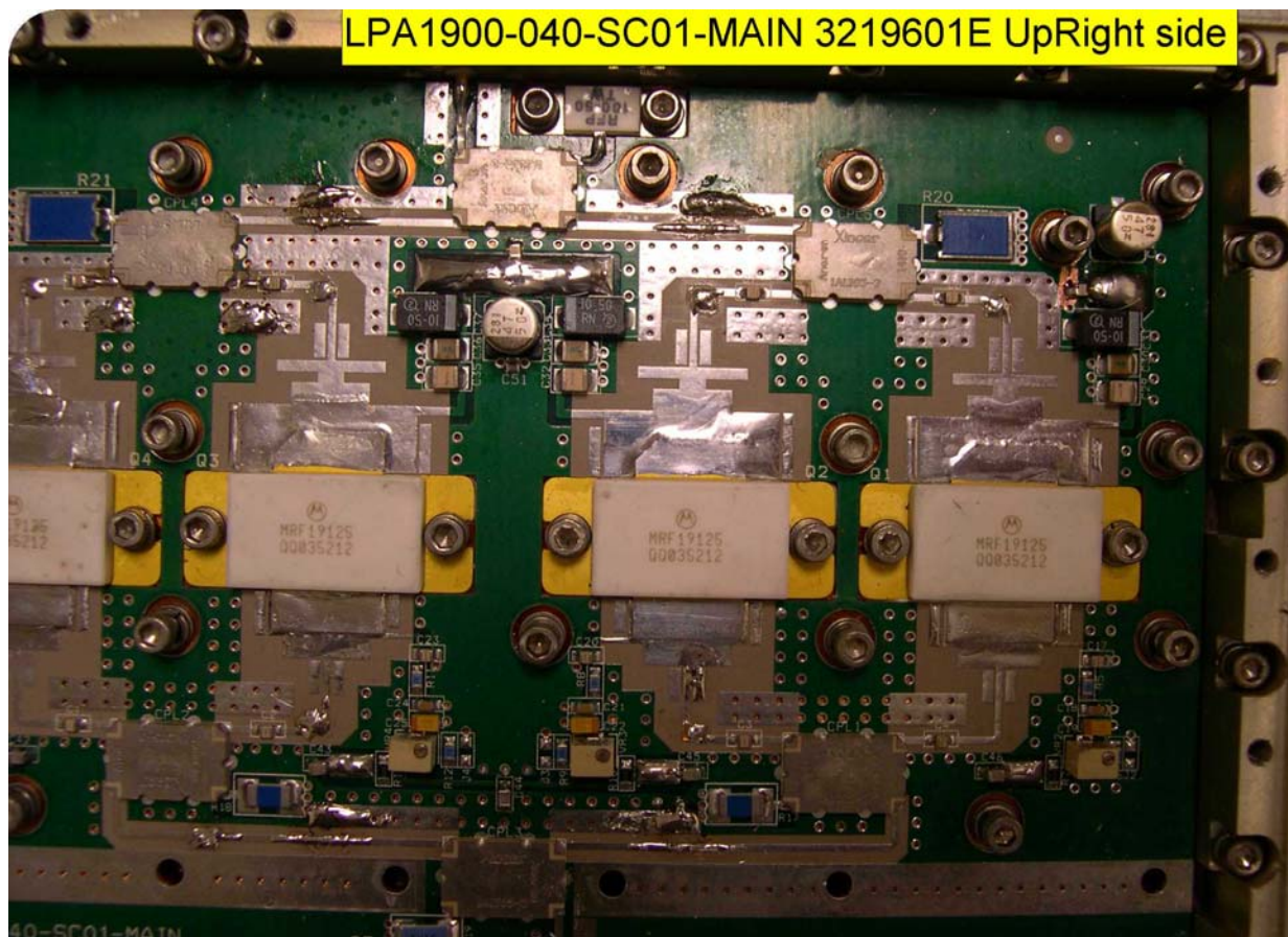
1900 MHz Linear Power Amplifier LPA1900-040-SC01-MAIN 3219601E UpRight
