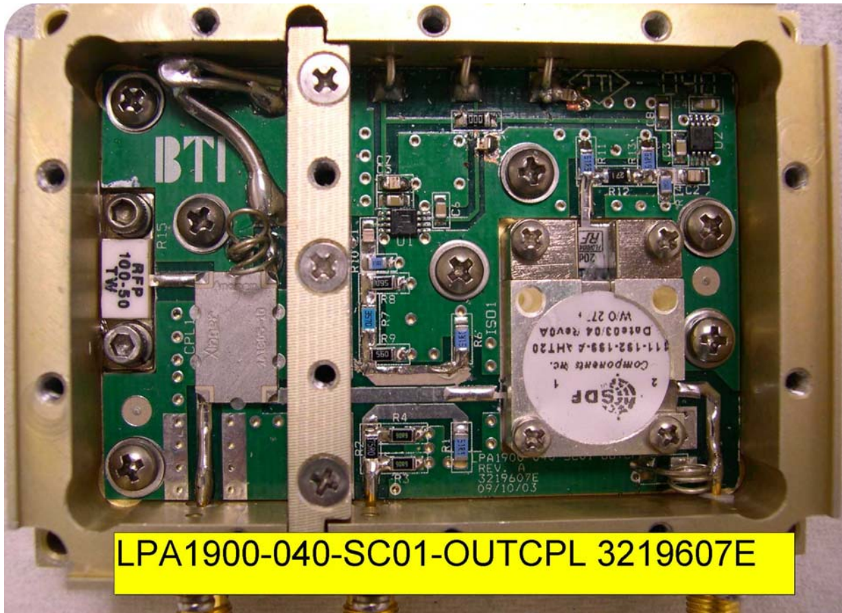
1900 MHz Linear Power Amplifier LPA1900-040-SC01-OUTCPL 3219607E
