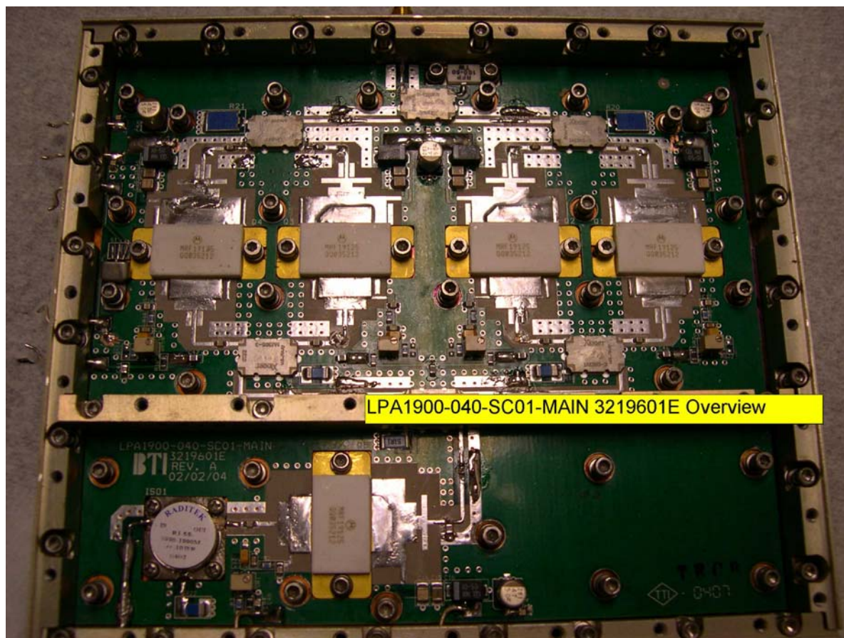
1900 MHz Linear Power Amplifier LPA1900-040-SC01-MAIN 3219601E Overview
