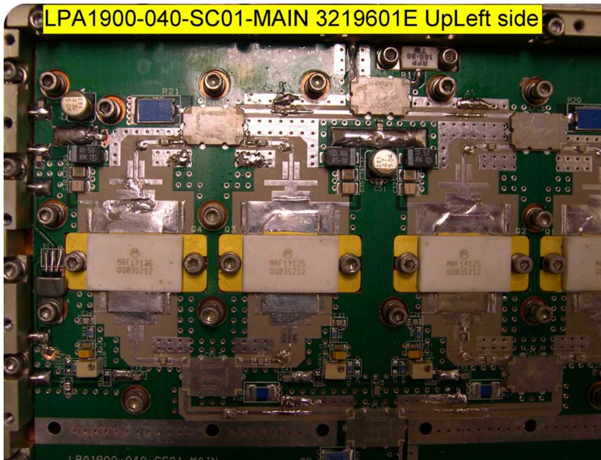
1900 MHz Linear Power Amplifier LPA1900-040-SC01-MAIN 3219601E UpLeft
