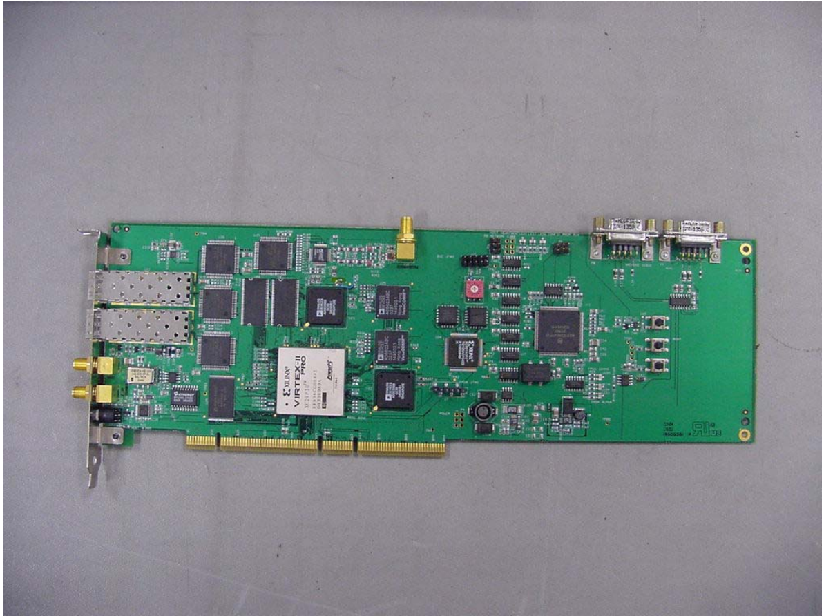
Software Defined Radio Card Top View
