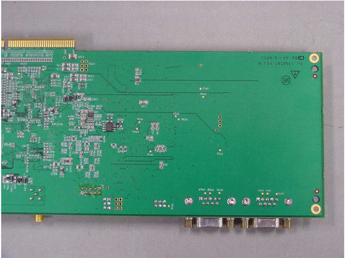
Software Defined Radio Card Bottom Right View
