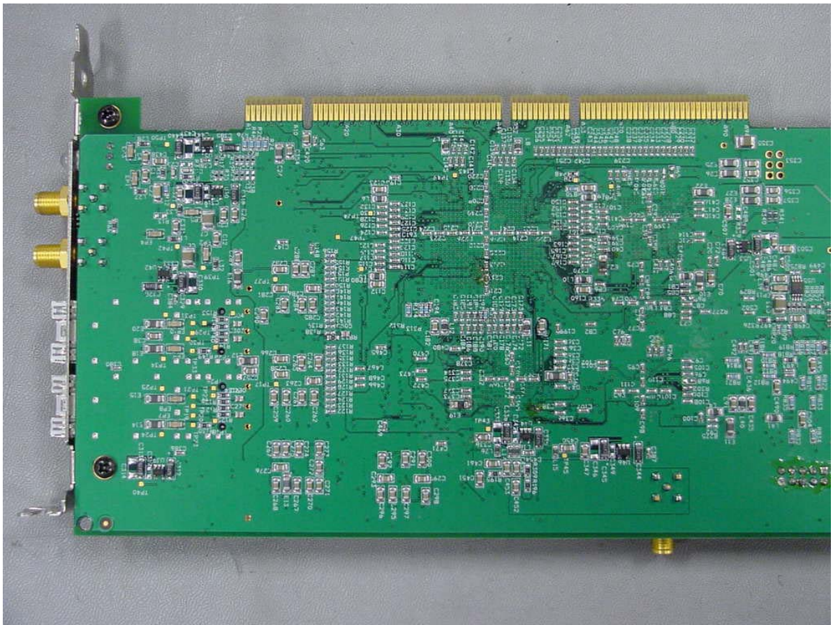
Software Defined Radio Card Bottom Left View
