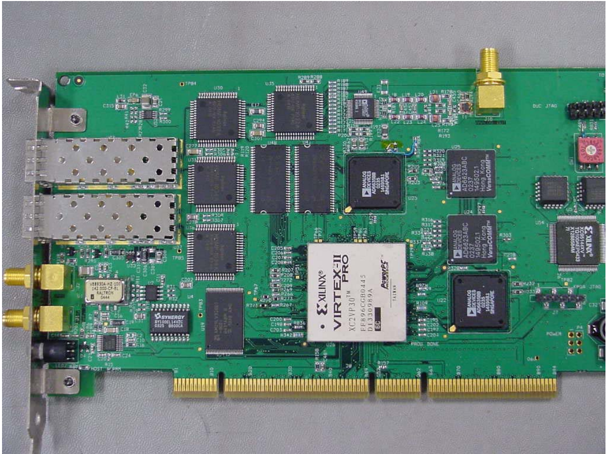
Software Defined Radio Card Top Left View
