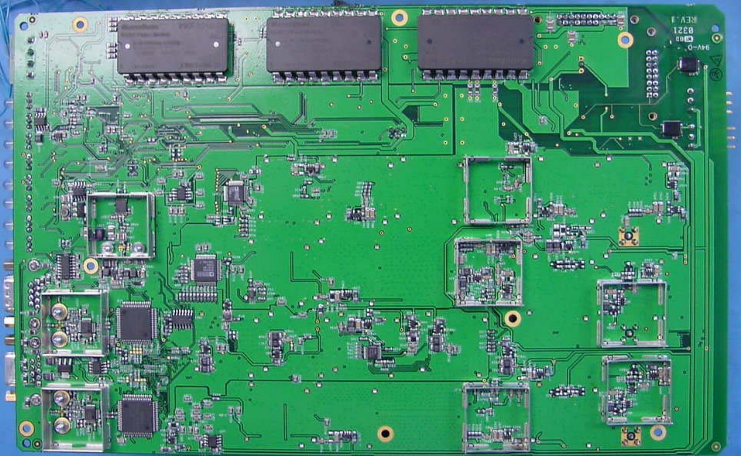
Digivance LRCS Signal Transport Module PCB Bottom View
