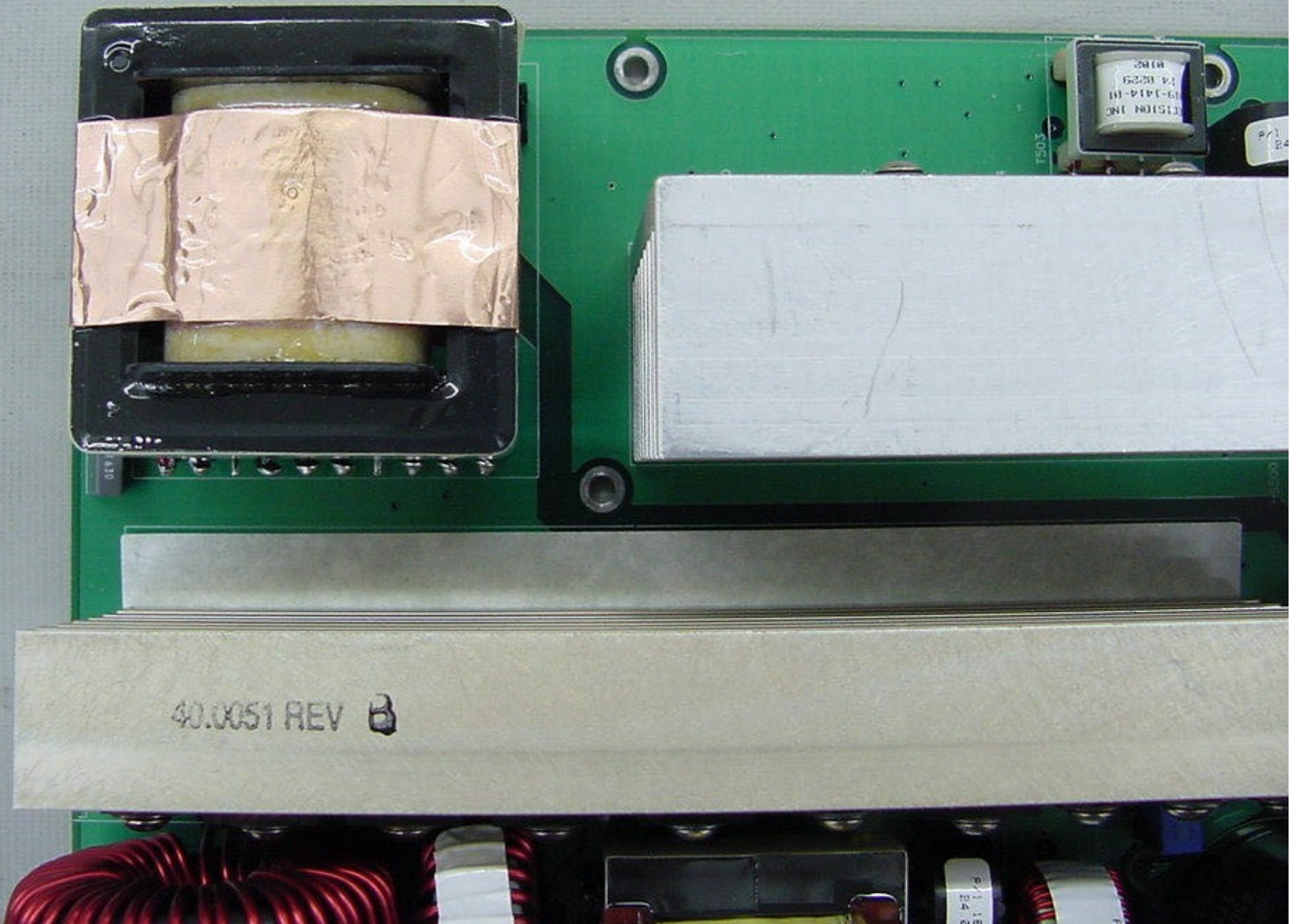
Wide Band Digital Radio 800 MHz Digivance LRCS Power Supply Board Top View - Upper Left
