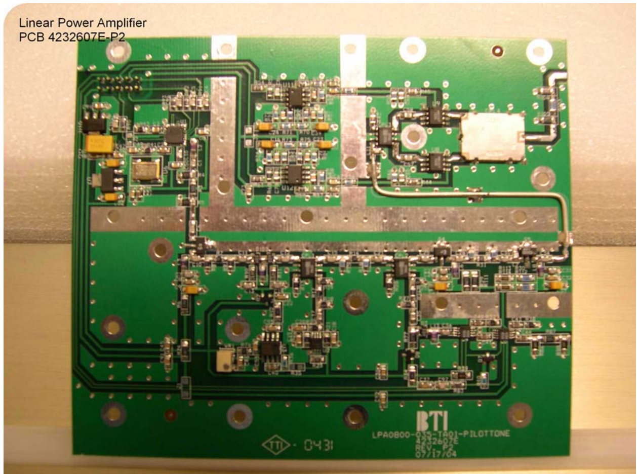
Linear Power Amplifier PCB 4232607E-P2 Back View
