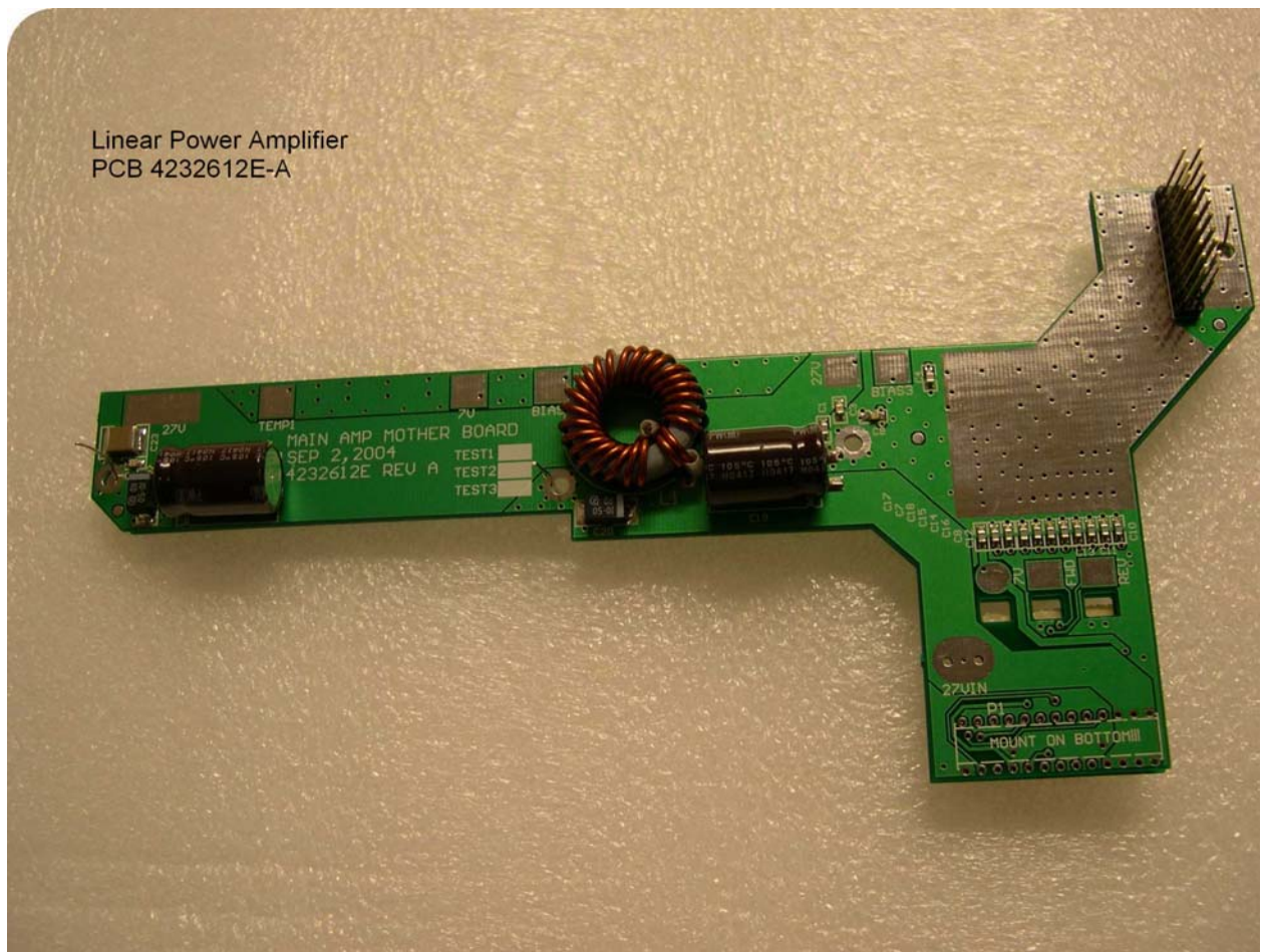
Linear Power Amplifier PCB 4232612E-A Back View
