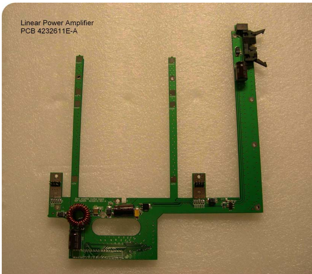
Linear Power Amplifier PCB 4232611E-A Back View
