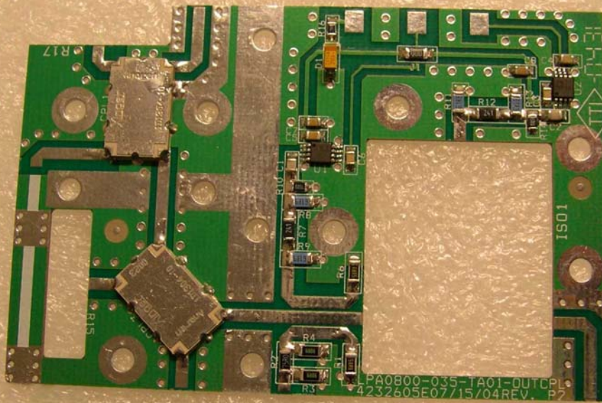
Linear Power Amplifier PCB 4232605E-P2
