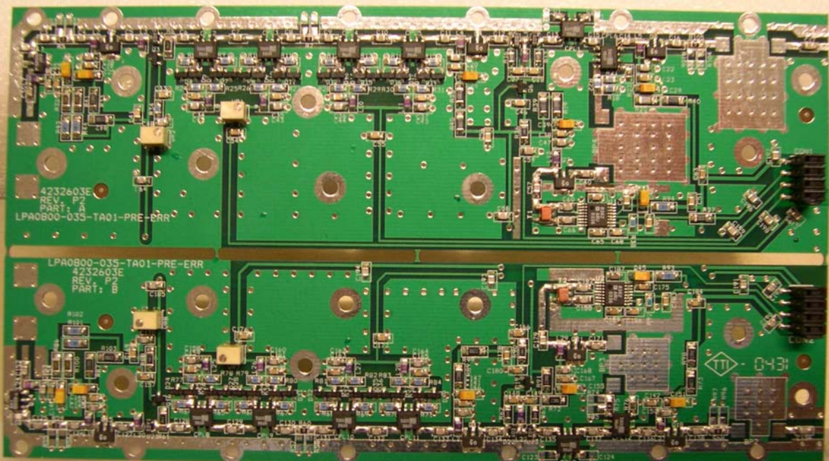
Linear Power Amplifier PCB 4232603E-P2
