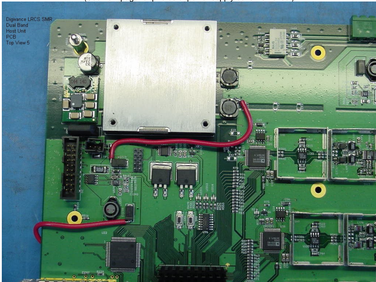
Digivance LRCS SMR Dual Band Host Unit PCB Top View 6
