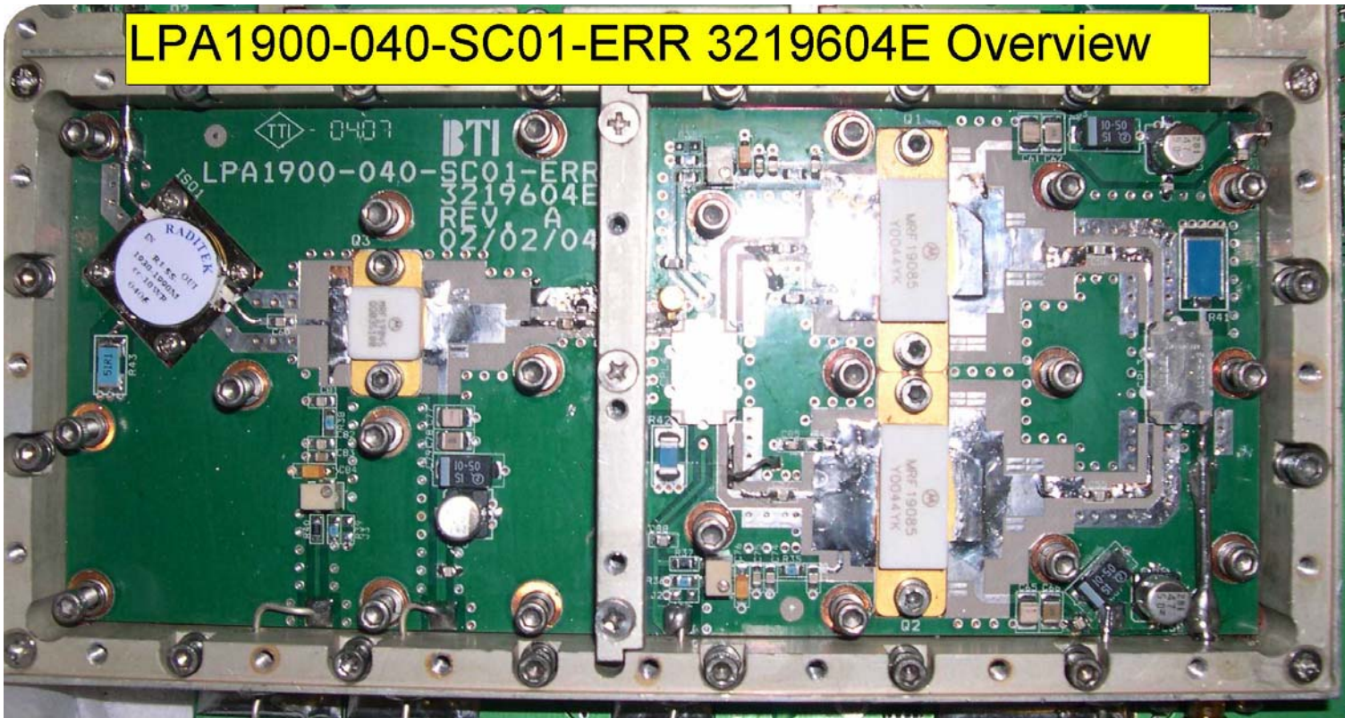
1900 MHz Linear Power Amplifier LPA1900-040-SC01-ERR 3219604E Overview
