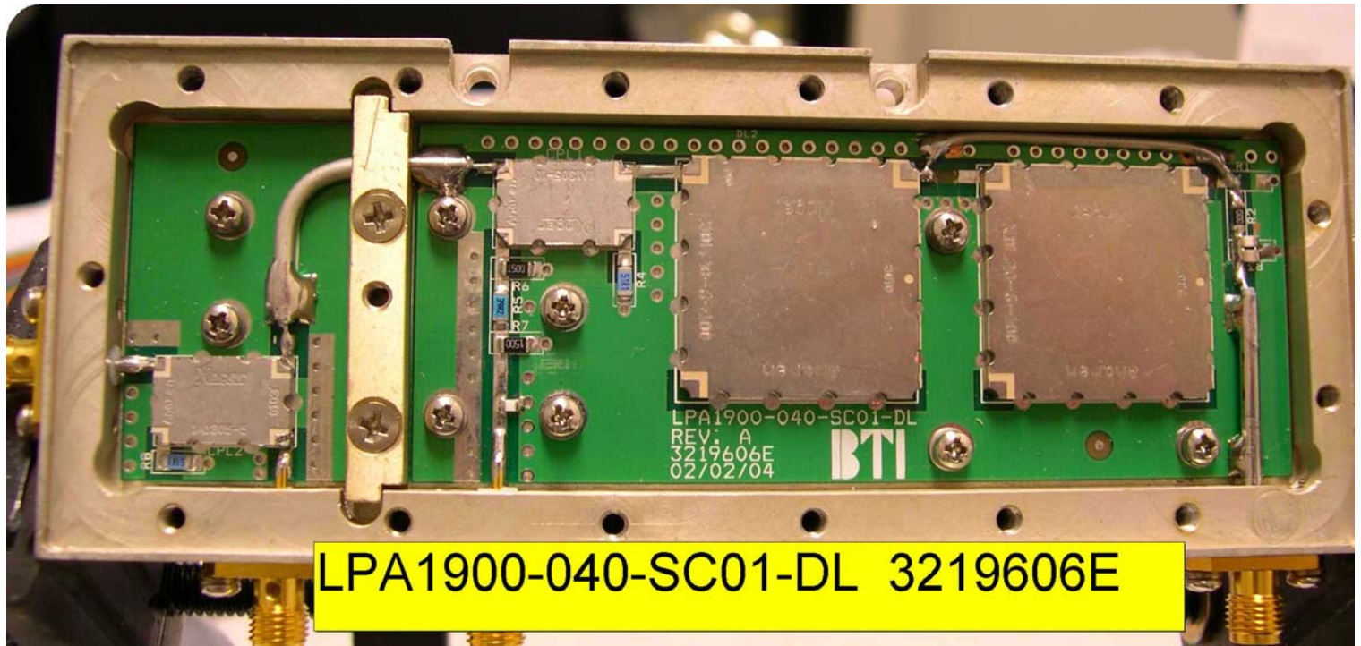
1900 MHz Linear Power Amplifier LPA1900-040-SC01 3219606E
