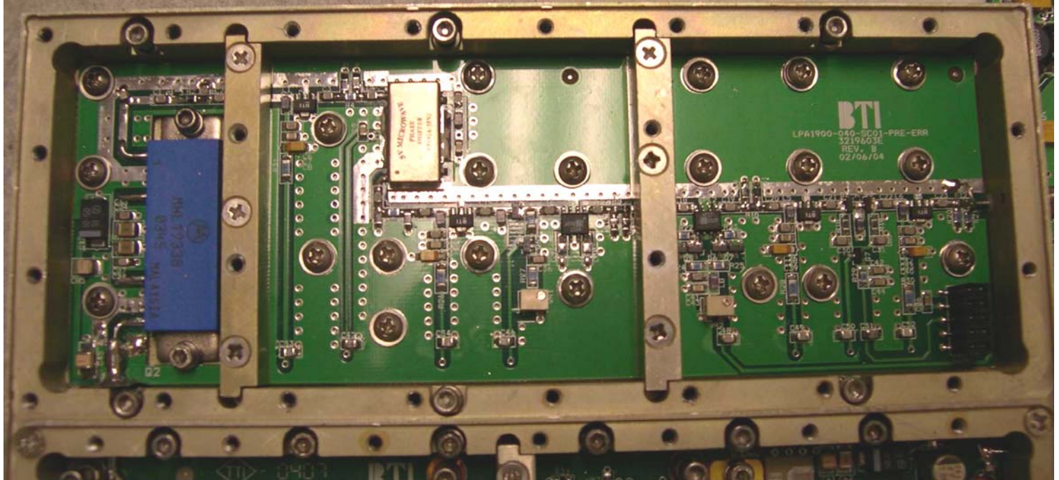
1900 MHz Linear Power Amplifier LPA1900-040- SC01-PRE-ERR 3219603E Overview
