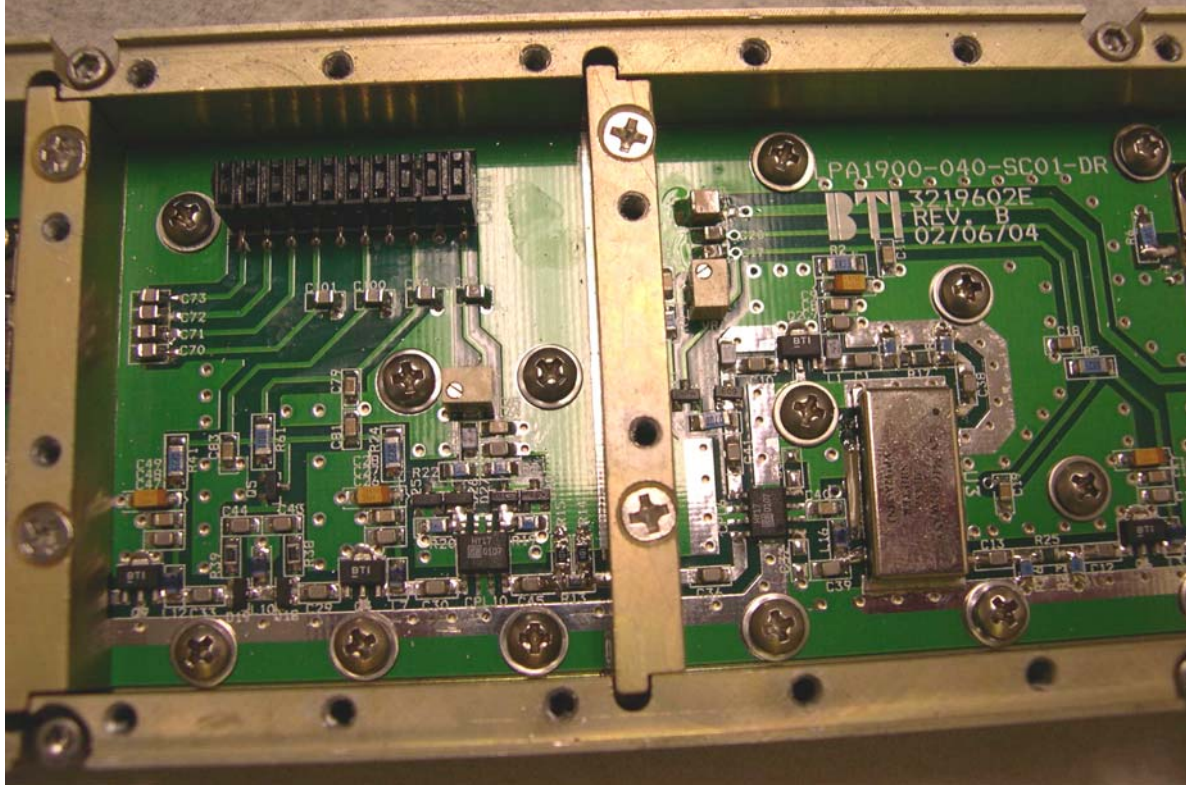
1900 MHz Linear Power Amplifier LPA1900-040-SC01-DR 3219602E LeftCenter
