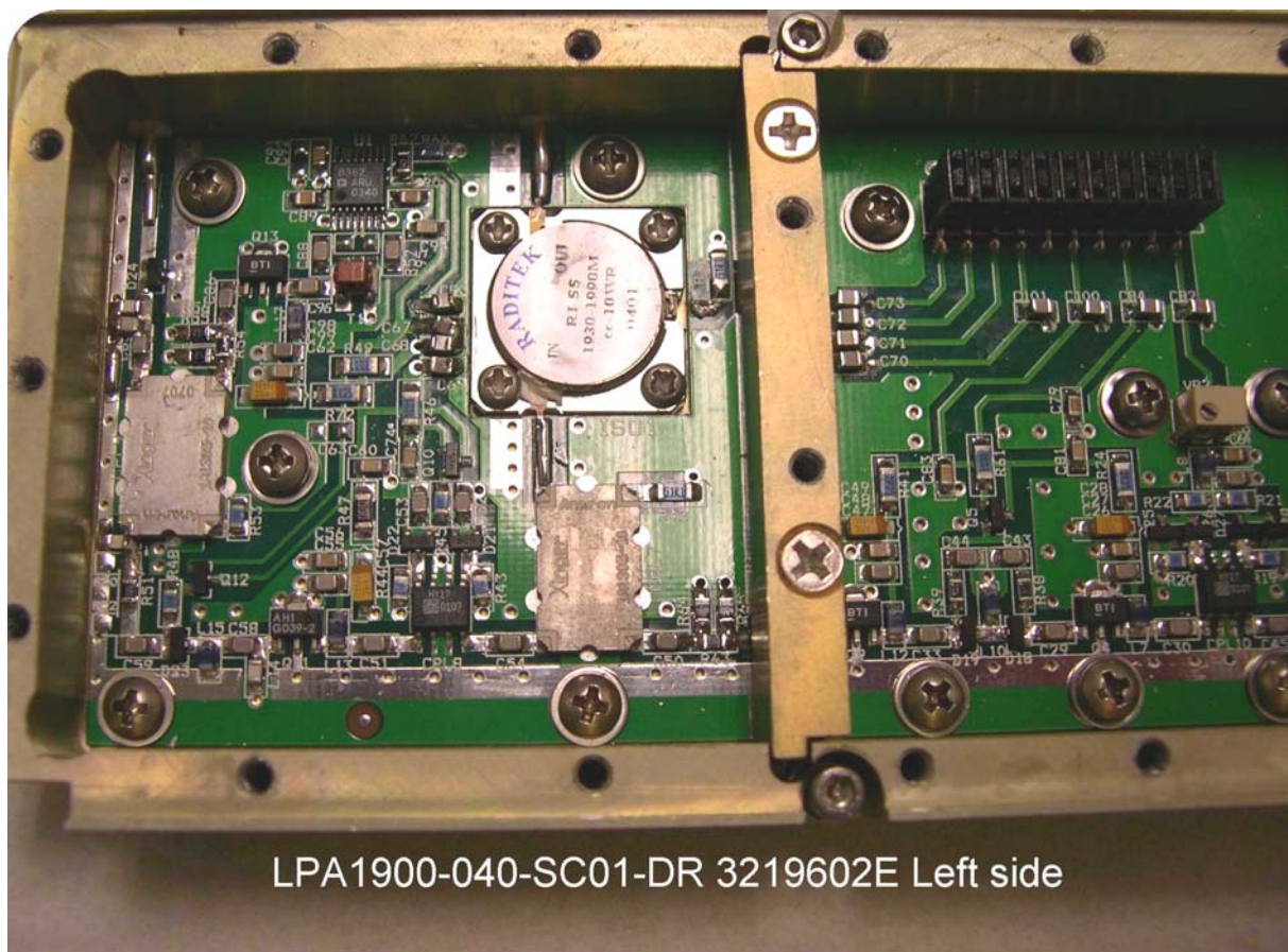
1900 MHz Linear Power Amplifier LPA1900-040-SC01-DR 3219602E Left
