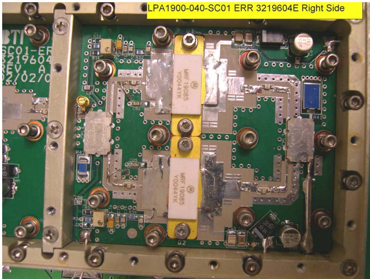
1900 MHz Linear Power Amplifier LPA1900-040-SC01-ERR 3219604E Right
