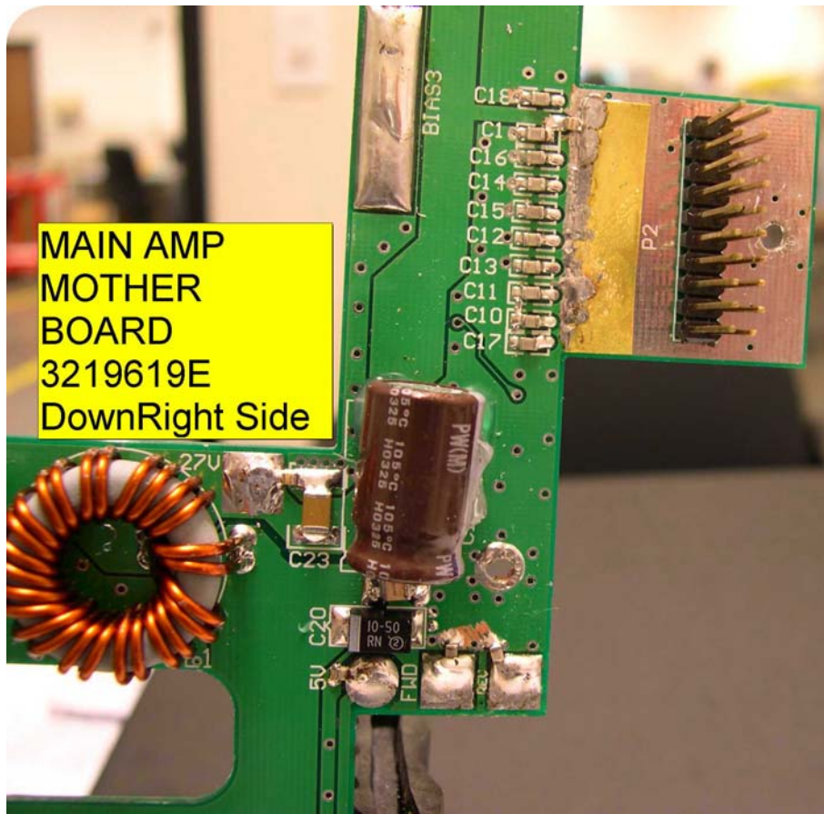
1900 MHz Linear Power Amplifier MAIN AMP MOTHER BOARD 3219619E DownRight
