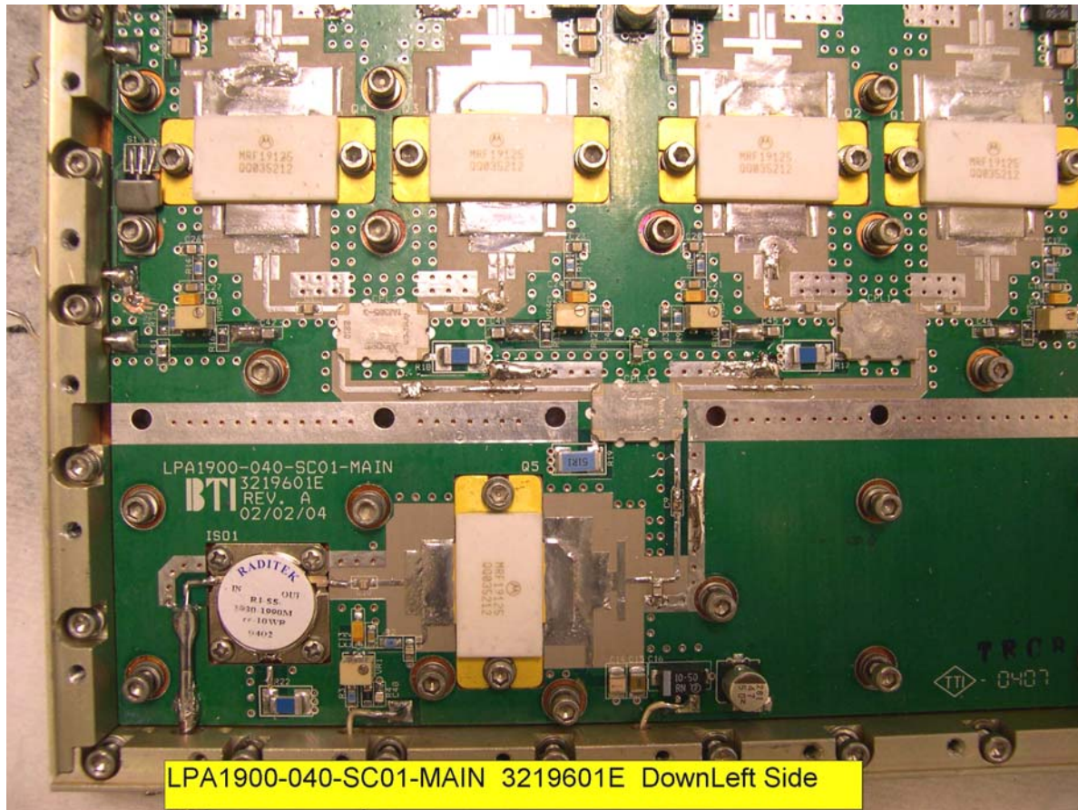
1900 MHz Linear Power Amplifier LPA1900-040-SC01-MAIN 3219601E DownLeft
