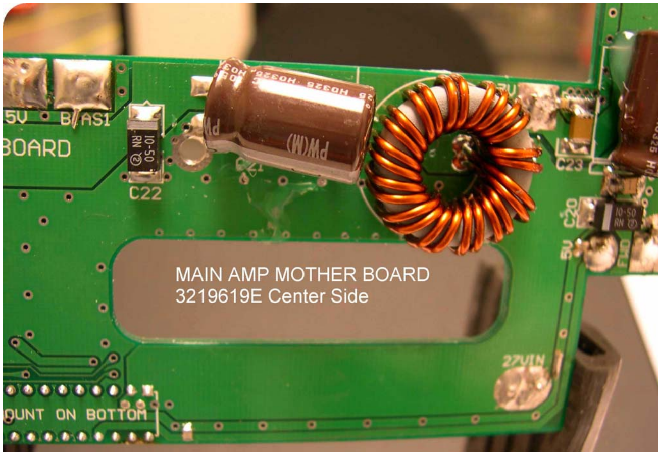
1900 MHz Linear Power Amplifier MAIN AMP MOTHER BOARD 3219619E Center
