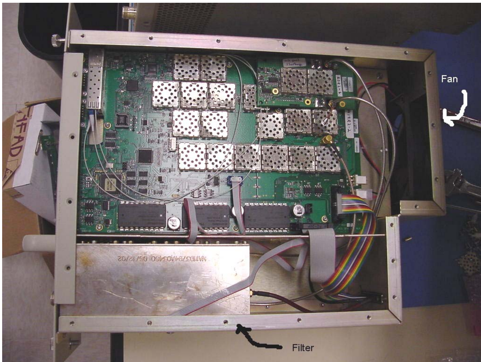
Digivance LRCS 1900 MHz Signal Transport Module – STM Open Right View
