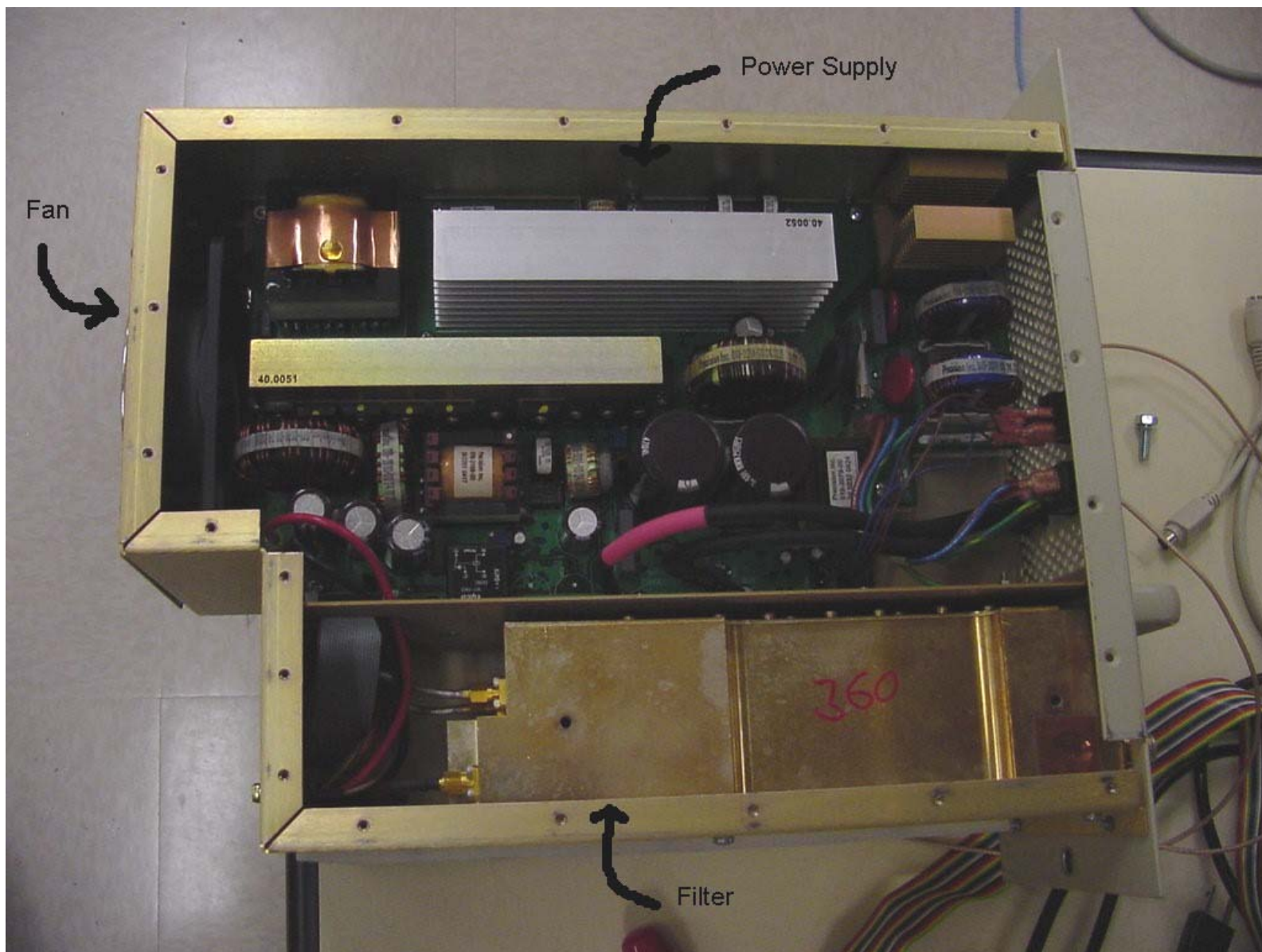
Digivance LRCS 1900 MHz Signal Transport Module – STM Open Left View
