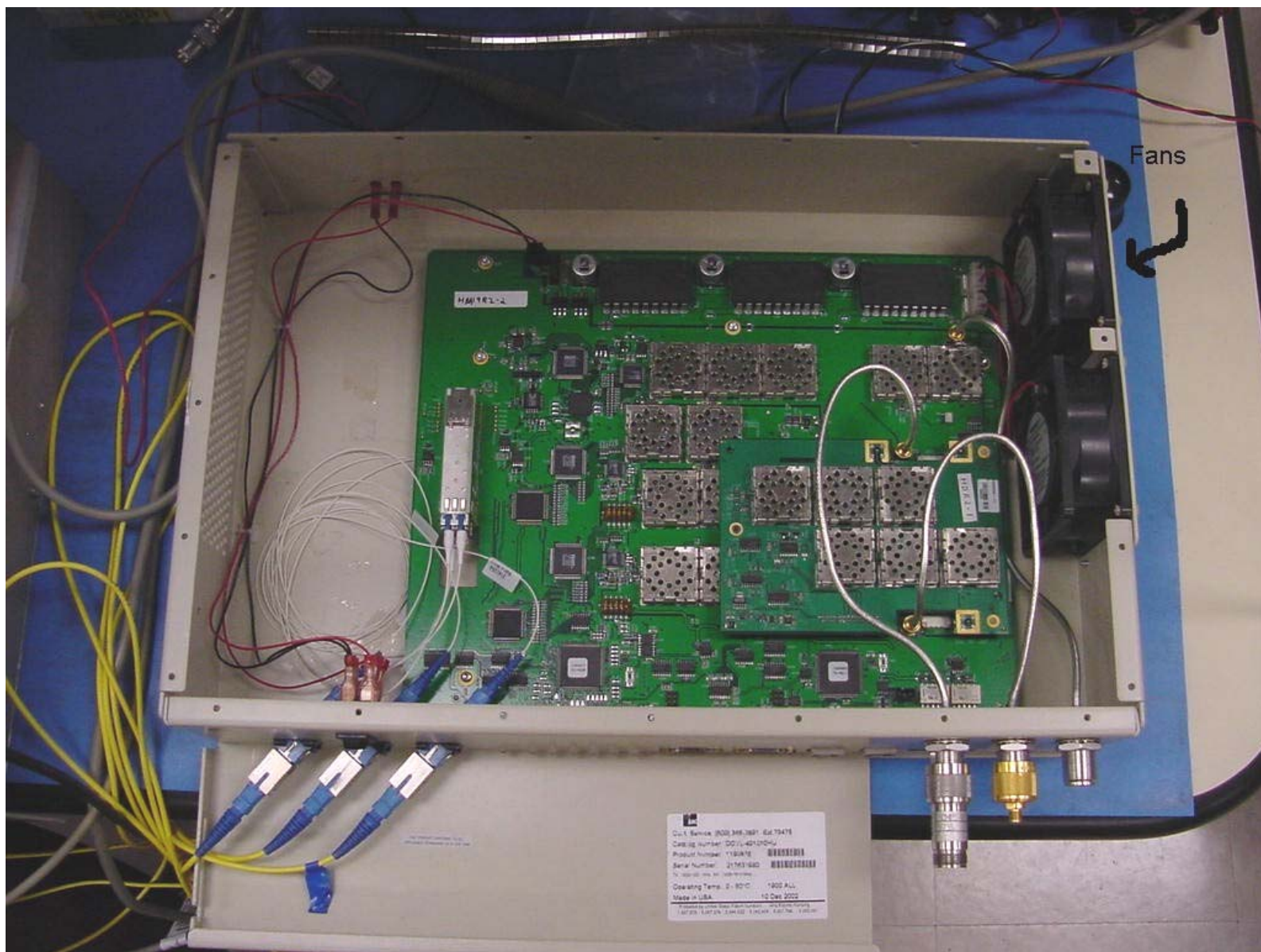
Digivance LRCS 1900 MHz Host Unit Open Top View
