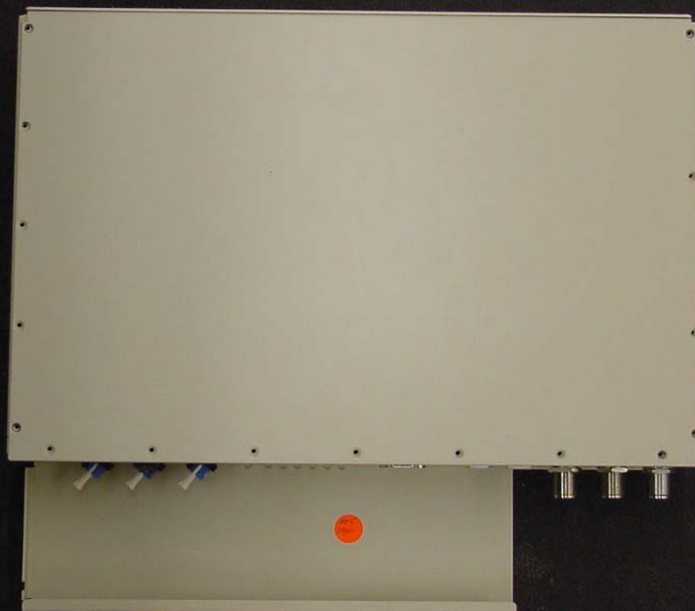
Digivance 1900 MHz LRCS Host Module Top View
