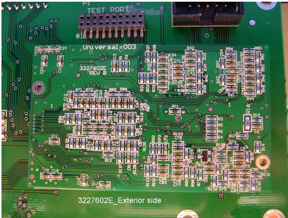
800 MHz Linear Power Amplifier 3227602E_ES
