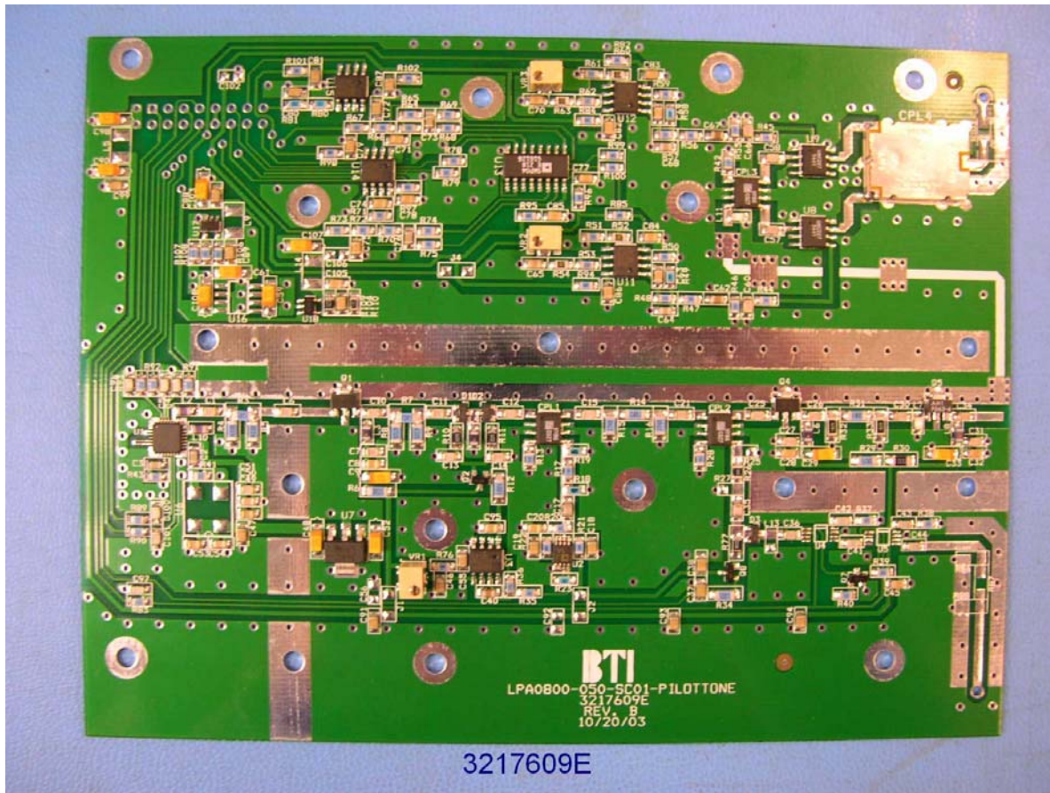
800 MHz Linear Power Amplifier 3217609E
