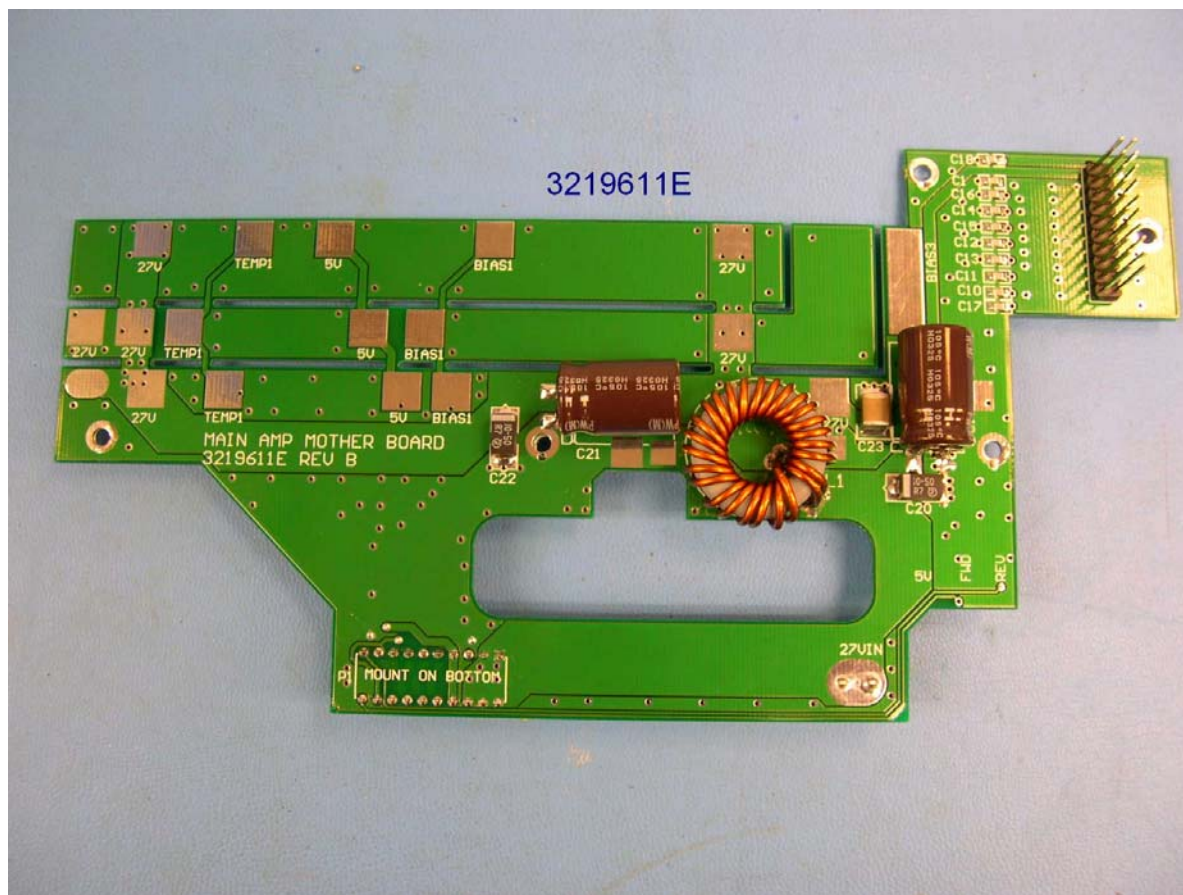
800 MHz Linear Power Amplifier 3219611E
