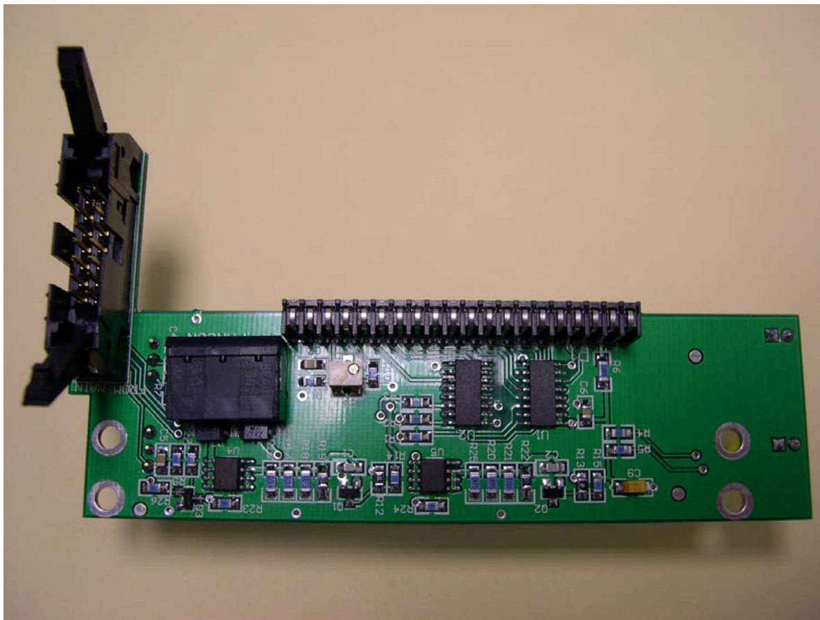
800 MHz Linear Power Amplifier 3219613E_Back
