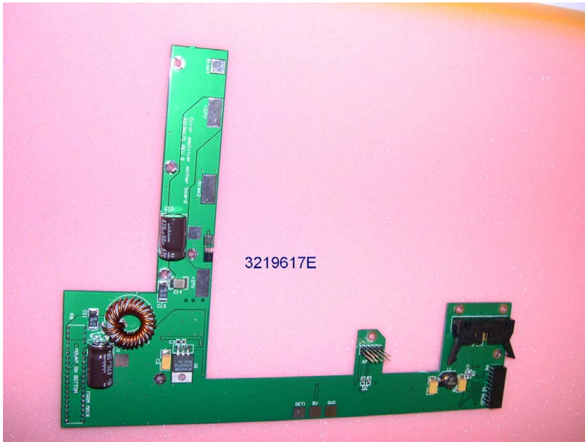
800 MHz Linear Power Amplifier 3219617E
