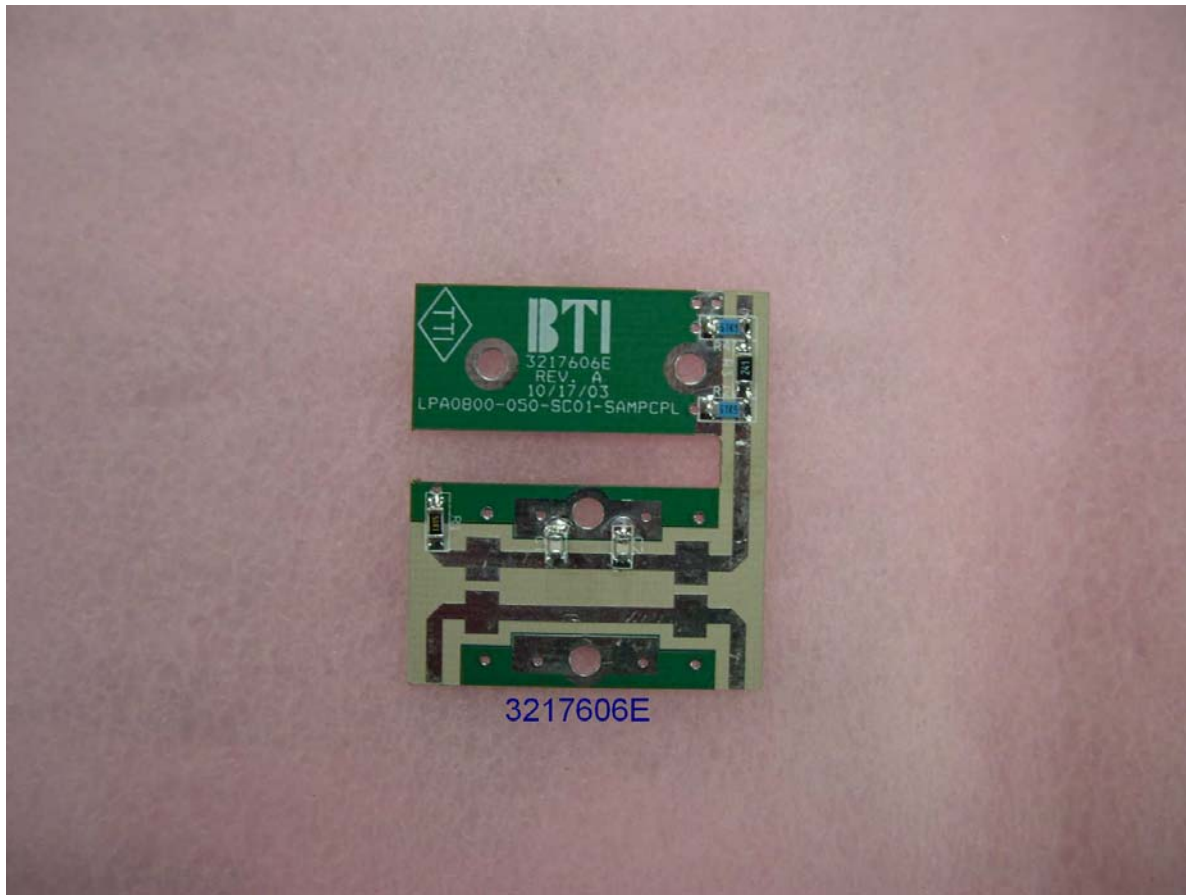
800 MHz Linear Power Amplifier 3217606E
