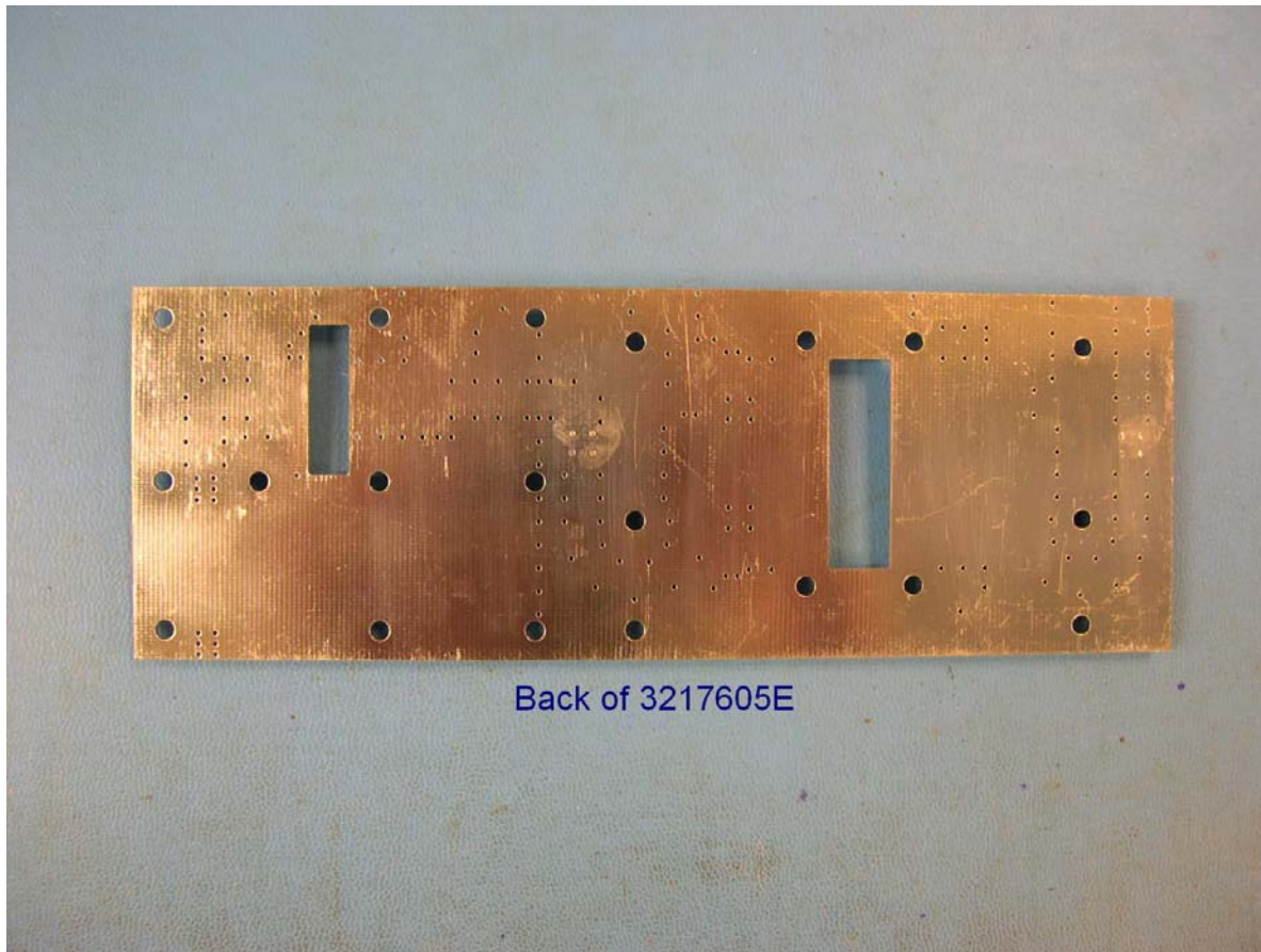
800 MHz Linear Power Amplifier 3217605E_Back
