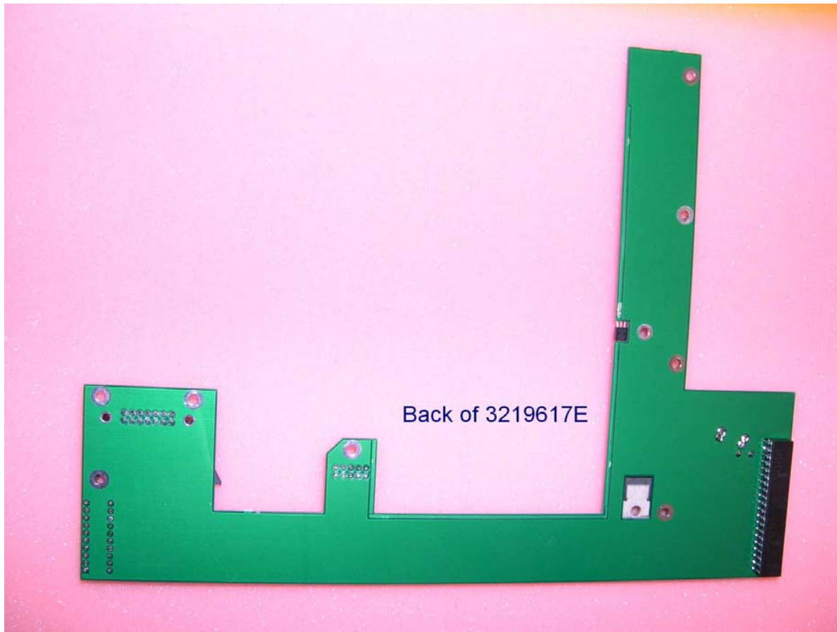
800 MHz Linear Power Amplifier 3219617E_Back
