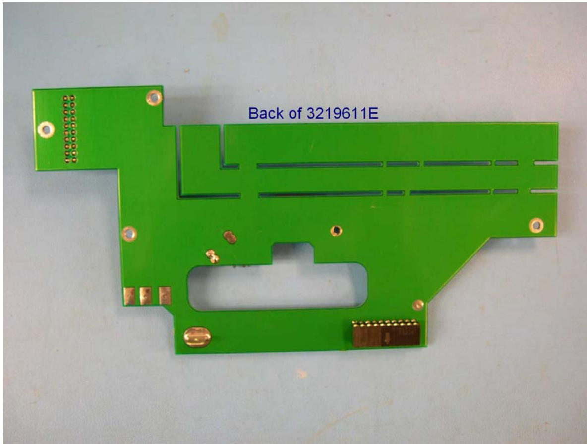
800 MHz Linear Power Amplifier 3219611E_Back
