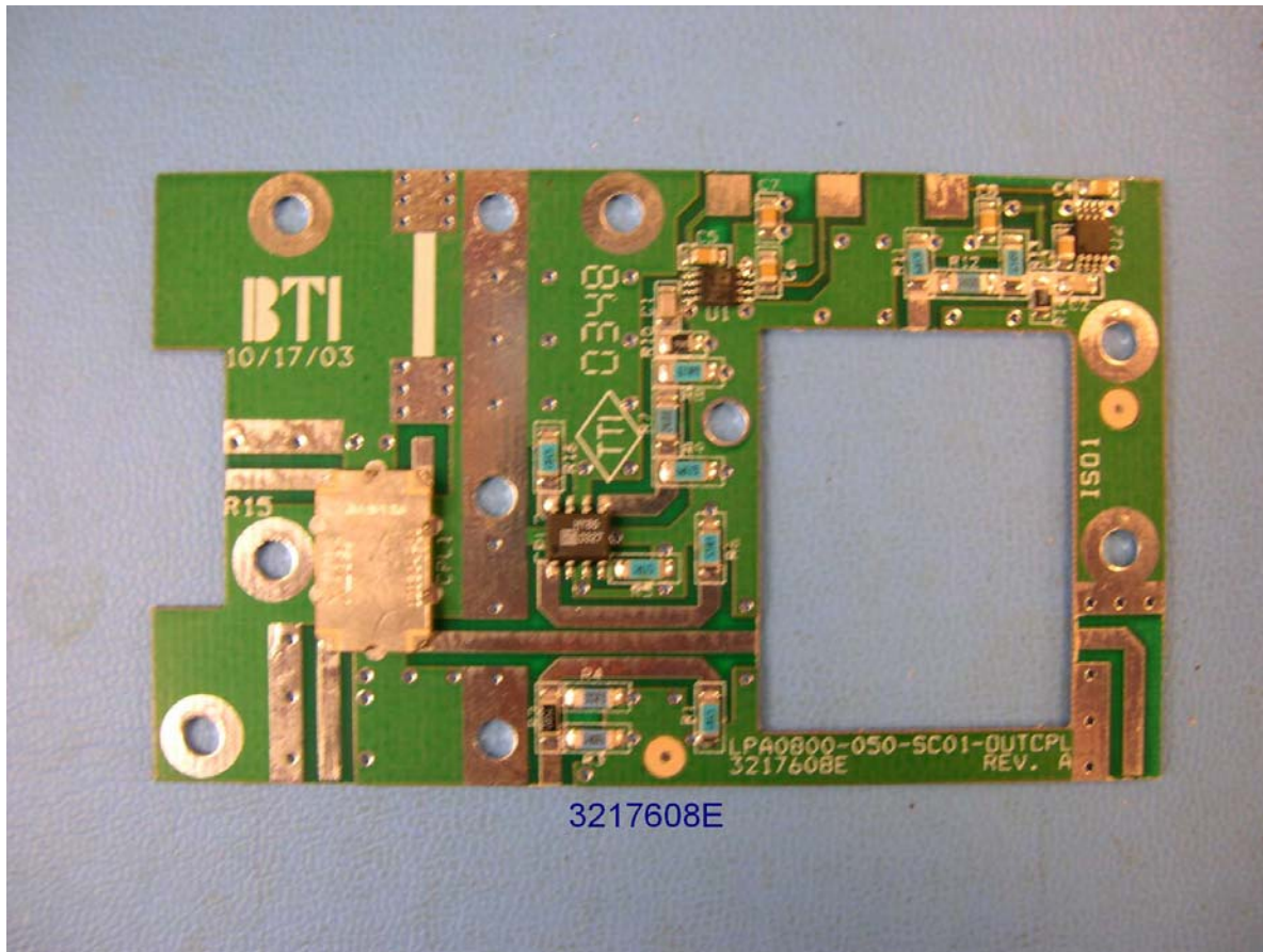
800 MHz Linear Power Amplifier 3217608E
