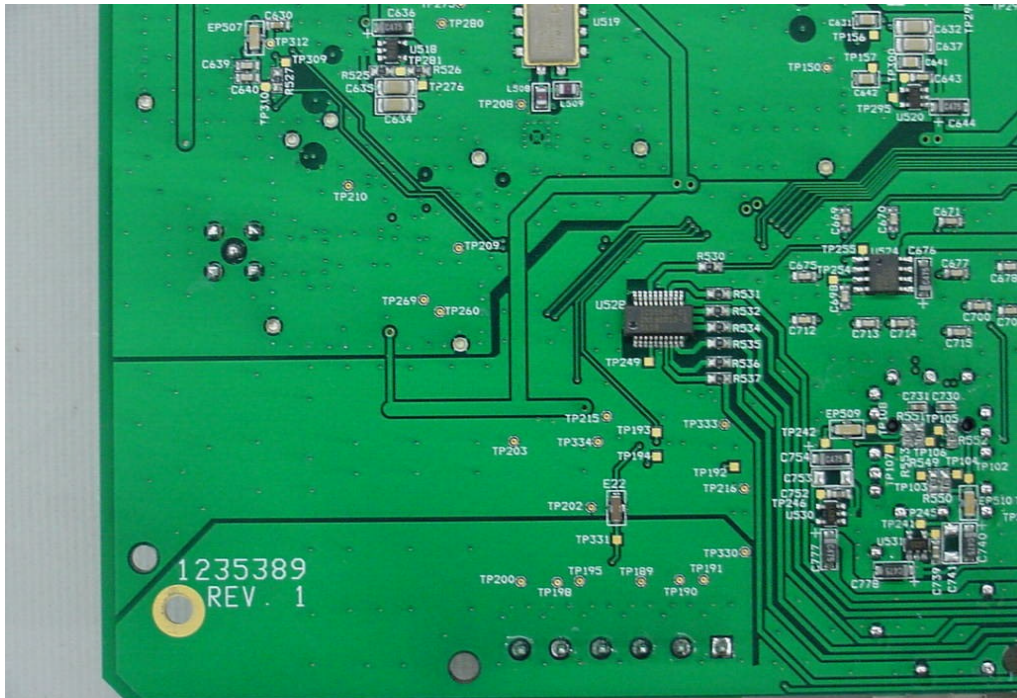
Digivance ICS SMR DHU Control Board - B1
