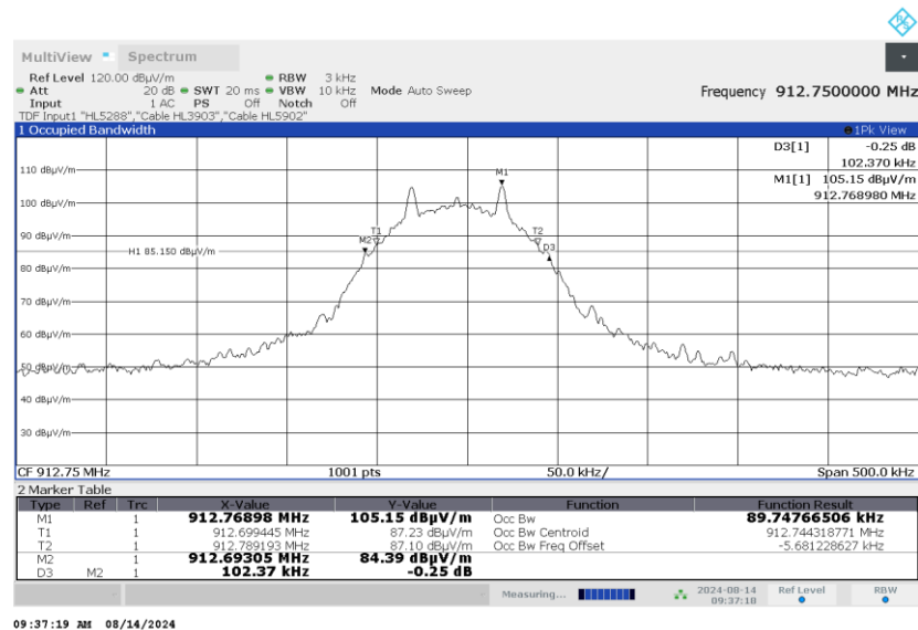
Plot 7.1.1 The 20 dB bandwidth test result at low frequency
