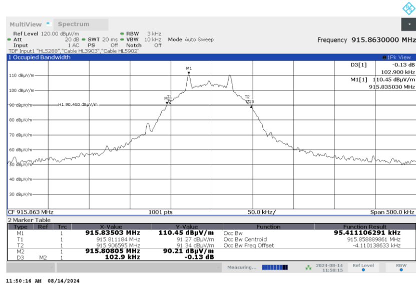
Plot 7.1.3 The 20 dB bandwidth test result at high frequency
