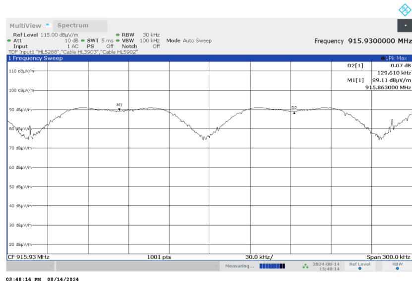
Plot 7.2.1 Carrier frequency separation
