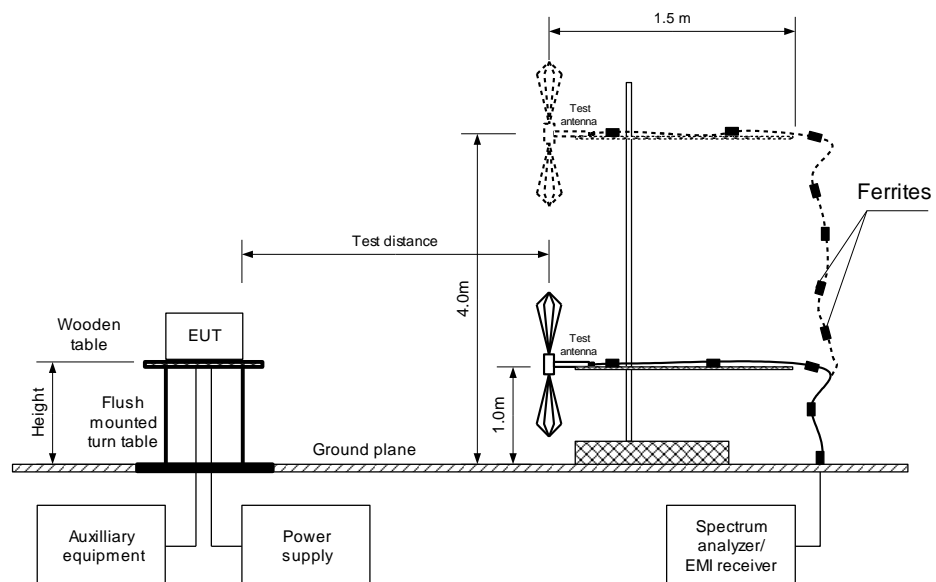
Figure 7.4.1 Average time of occupancy test setup
