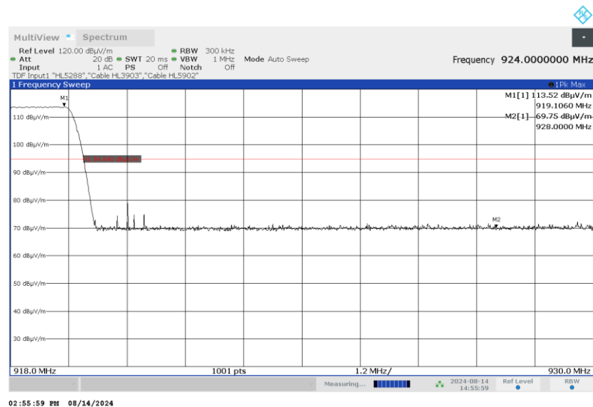
Plot 7.7.4 The highest band edge emission at high carrier frequency with hopping function enabled
