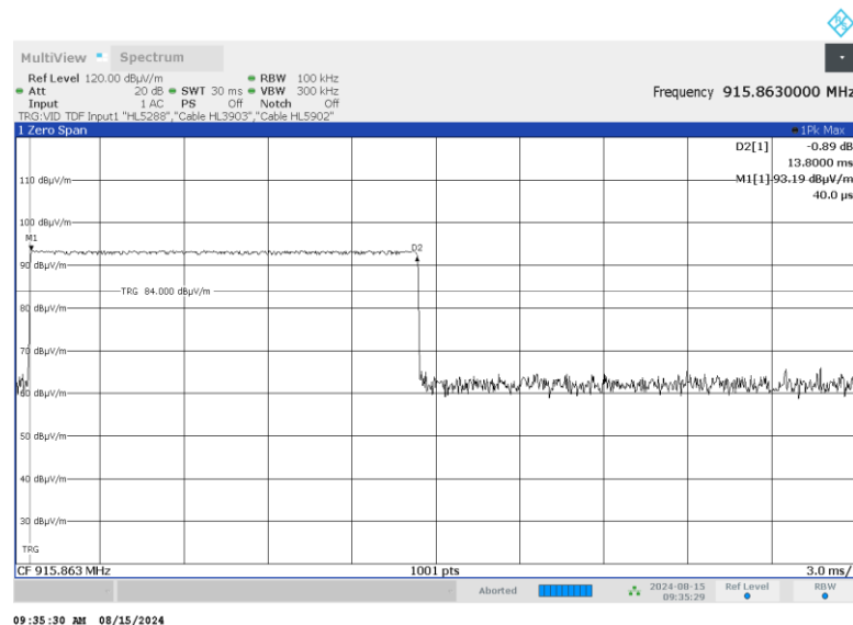
Plot 7.4.1 Single transmission duration
