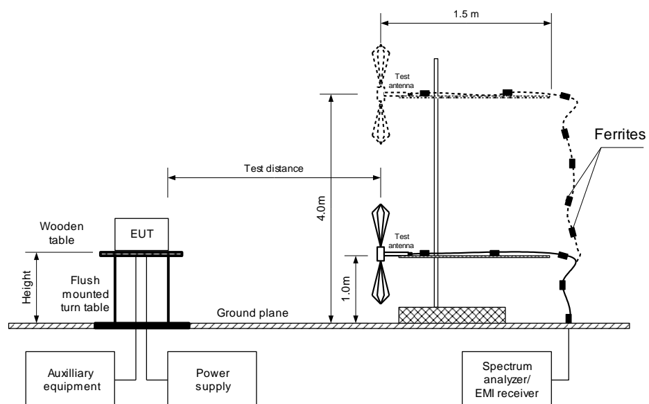
Figure 7.3.1 Hopping frequencies test setup
