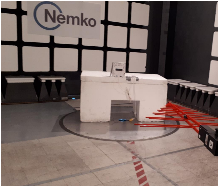
Radiated spurious (out-of-band) emissions setup photo – 30 to 1000 MHz
