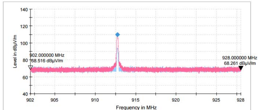
Plot 7.6.2 Radiated emission measurements at the mid carrier frequency
