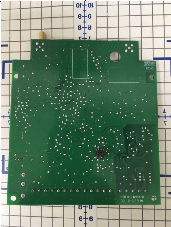
Host - Board Rear View
