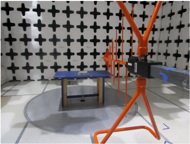
Spurious Emission Below 1GHz-Rear View
