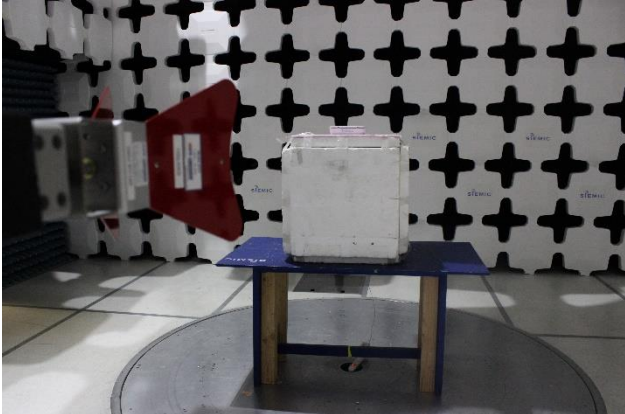
Spurious Emission Above 1GHz-Rear View
