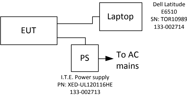
Figure 3.6-1: Setup diagram
