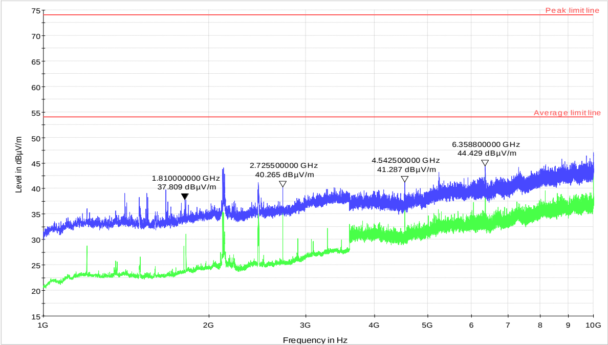
Figure 8.5-2: Field strength of spurious emissions above 1000 MHz
