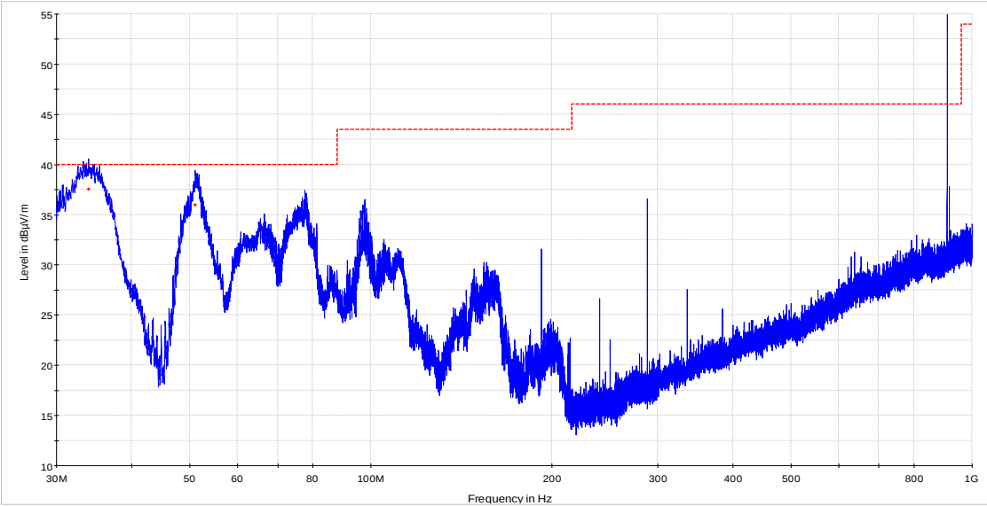
Figure 8.5-1: Field strength of spurious emissions below 1000 MHz
