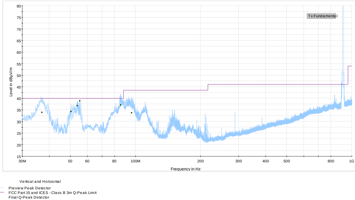
Figure 8.1-1: Radiated spurious emissions spectral plot – 30 to 1000 MHz
