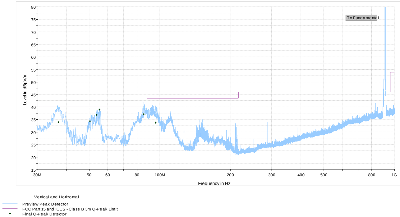
Figure 8.1-1: Radiated spurious emissions spectral plot – 30 to 1000 MHz
