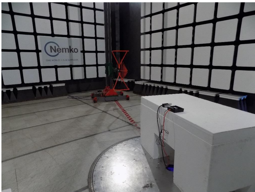
Figure 8.1-2: Radiated spurious (out-of-band) emissions setup photo – 30 to 1000 MHz
