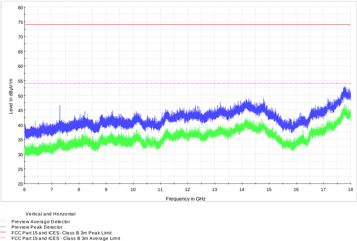
Figure 8.1-3: Radiated spurious emissions spectral plot – 6 to 18 GHz
