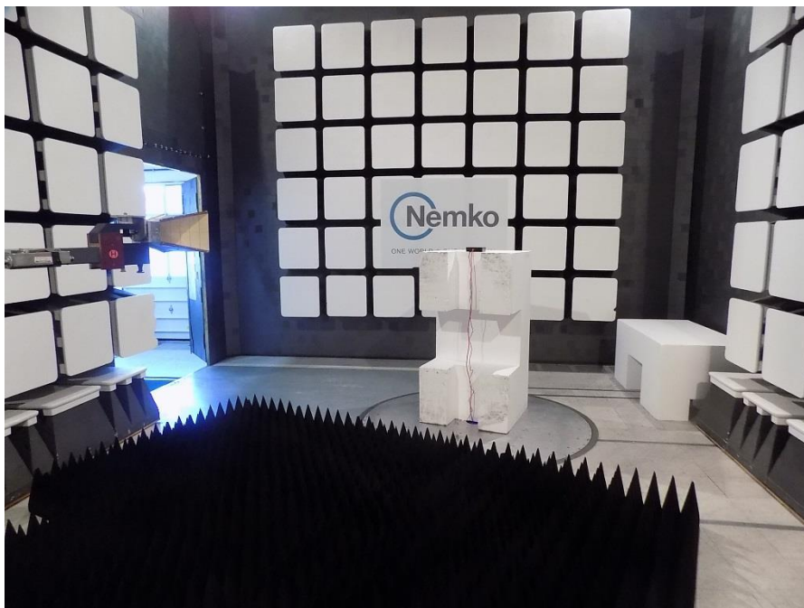
Figure 8.1-3: Radiated spurious (out-of-band) emissions setup photo – above 1 GHz
