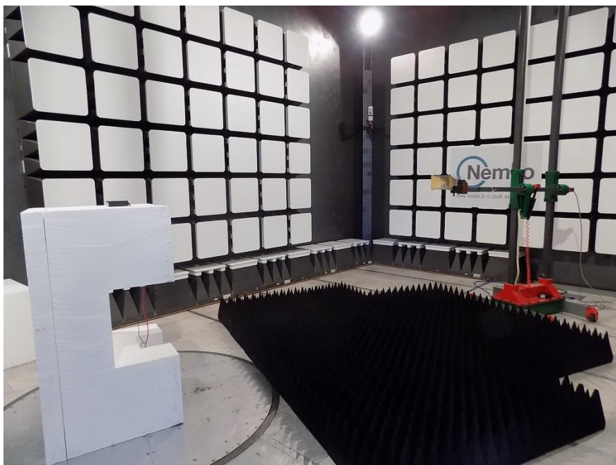
Figure 8.1-4: Radiated spurious (out-of-band) emissions setup photo – above 1 GHz
