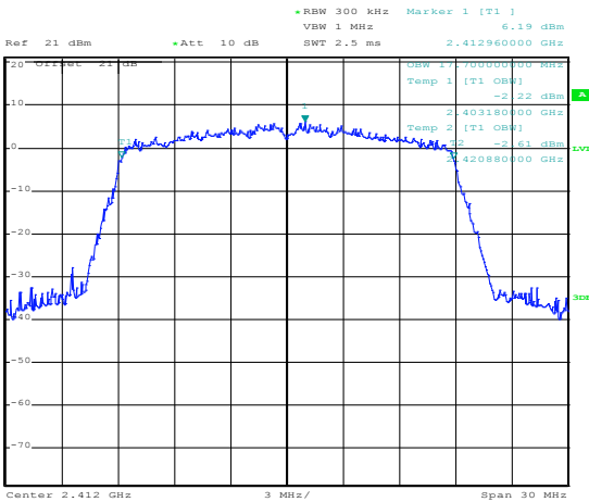
Figure 8.2-22: 99% bandwidth on 802.11n HT20, sample plot – QAM 64_3/4_65Mbps
