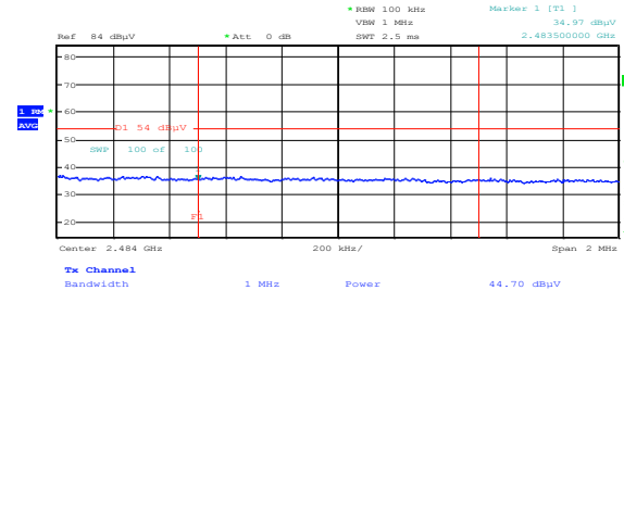
Figure 8.4-49: Radiated spurious emissions Upper band edge for 802.11n HT20, (TX 2462 MHz) – Average
