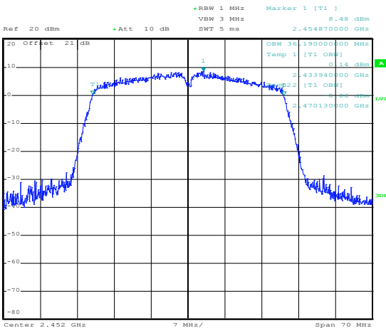
Figure 8.2-24: 99% bandwidth on 802.11n HT40, sample plot – OFDM: QAM 64_3/4_65Mbps
