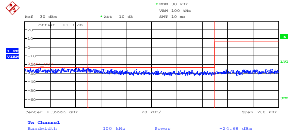
Figure 8.4-18: Conducted spurious emissions Lower band edge for 802.11b, (TX 2417 MHz)
