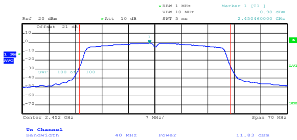
Figure 8.3-8: Conducted output power on 802.11n HT40, sample plot – QAM 64_3/4_65Mbps
