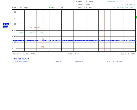
Figure 8.4-53: Radiated spurious emissions Upper band edge for 802.11b, (TX 2457 MHz) – Average
