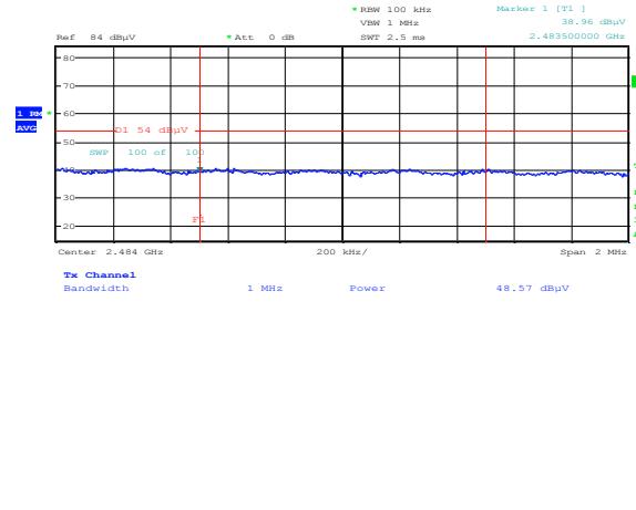
Figure 8.4-55: Radiated spurious emissions Upper band edge for 802.11g, (TX 2457 MHz) – Average
