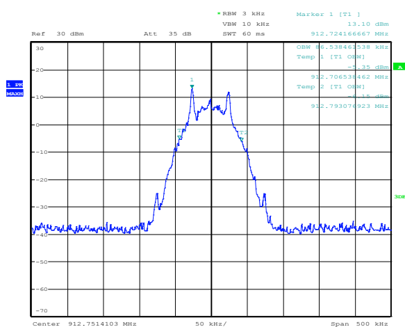
Figure 8.2-2: 20 dB bandwidth on mid channel
