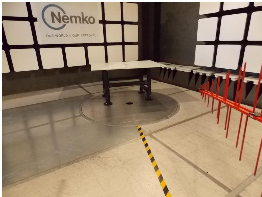
Figure 8.2-3: Emissions setup photo
