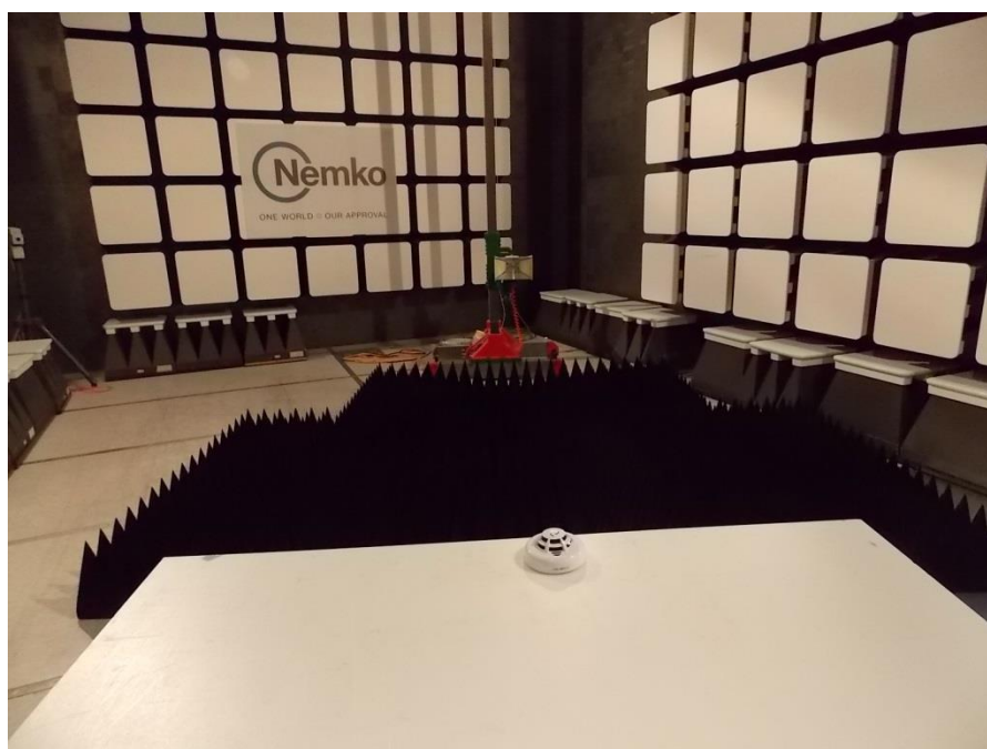
Figure 8.2-4: Emissions setup photo
