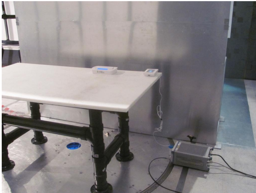
Photo 8.1-1: Conducted emissions setup
