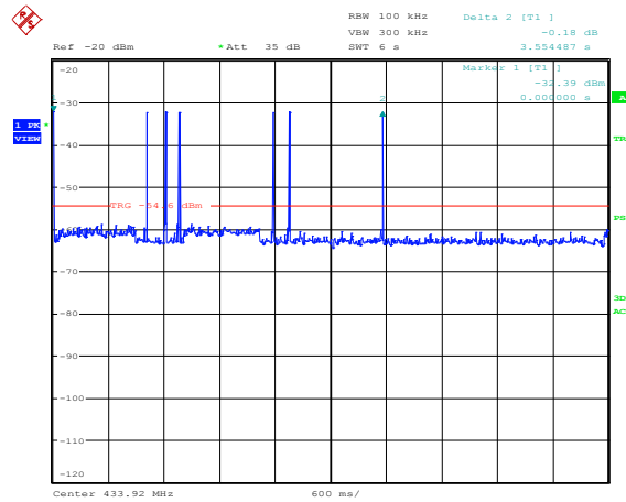
Plot 8.2-2: Automatic transmissions
