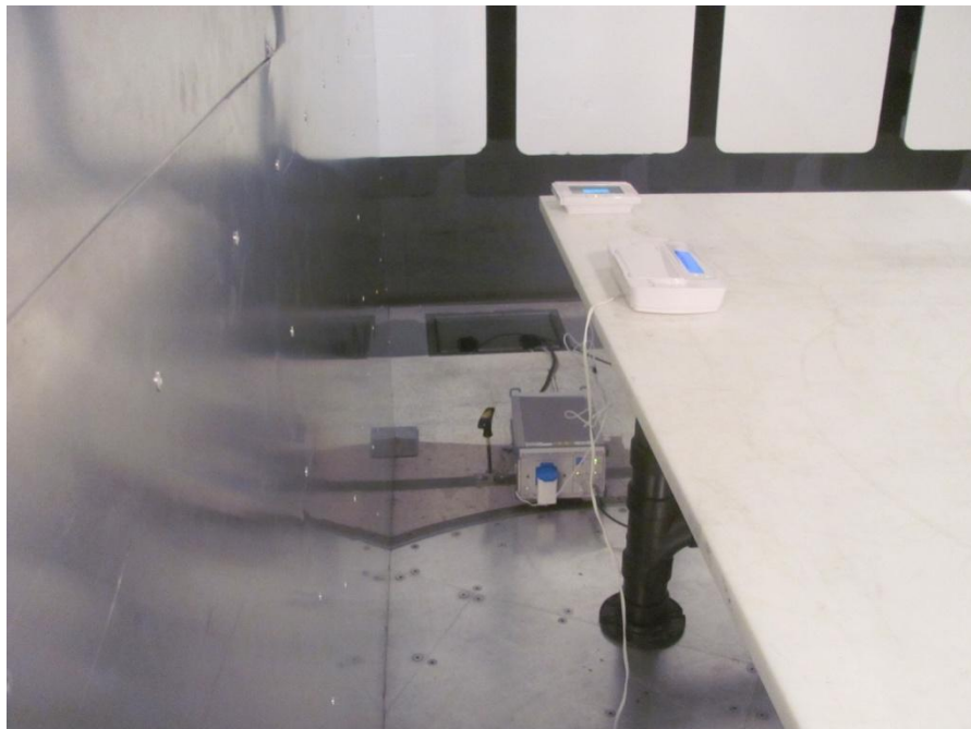
Photo 8.1-2: Conducted emissions setup
