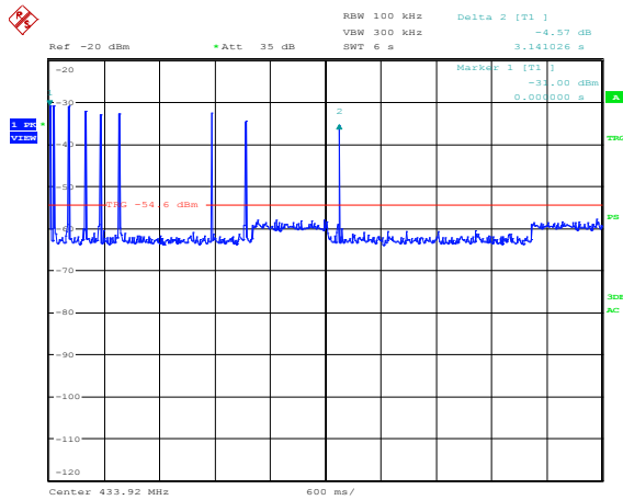
Plot 8.2-1: Manual transmissions
