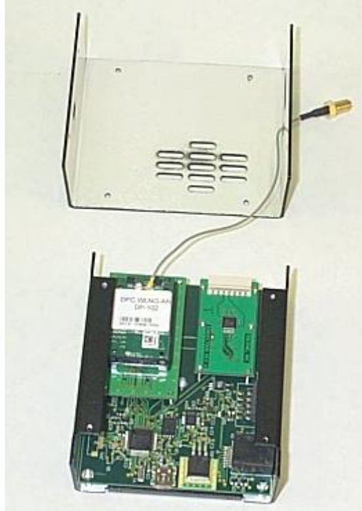
Photograph of Host Unit: Top Cover Removed
