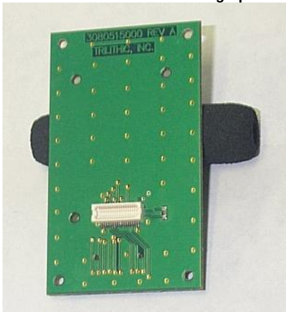
Component side
