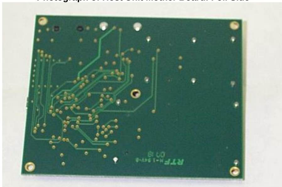
Photograph of Host Unit Mother Board: Foil Side
