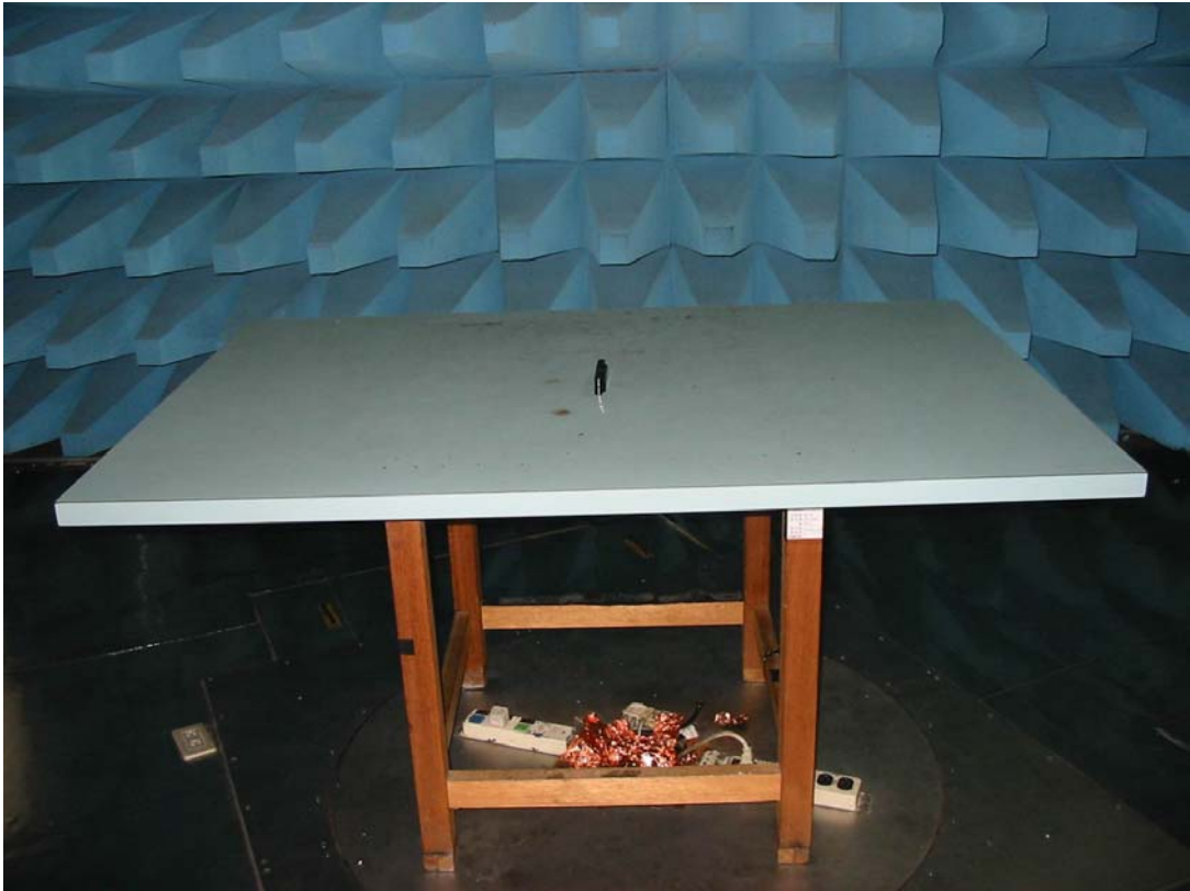
Front View of the Test Configuration of Y-plane
