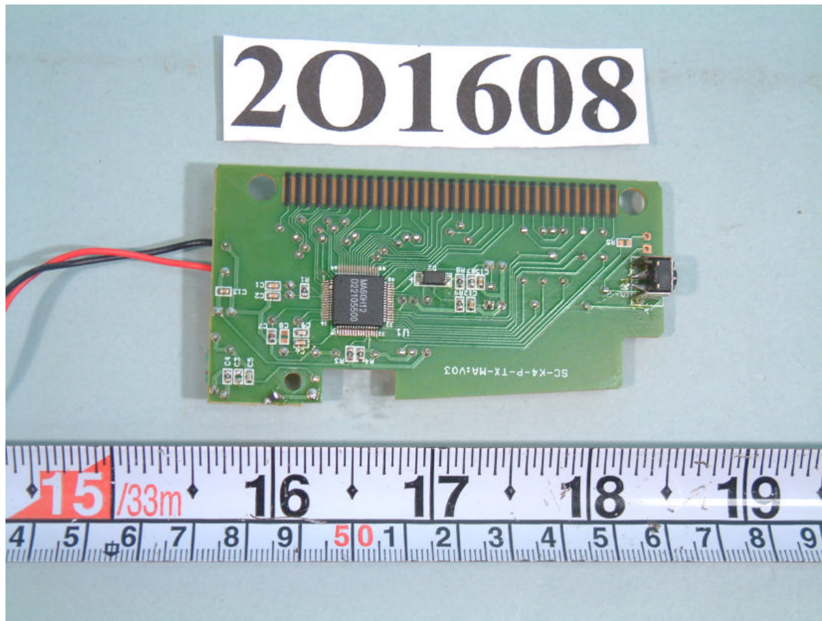
REAR side of Main Board(KEYBOARD)
