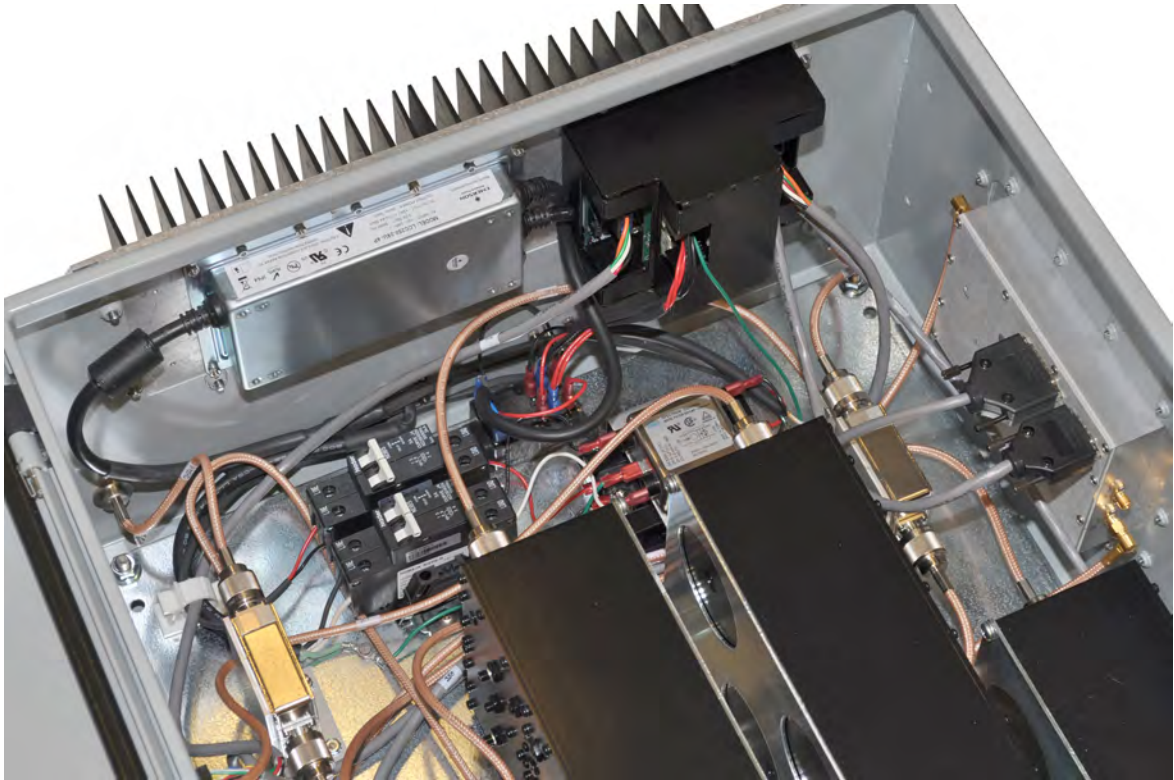
Enclosure close-up view.
