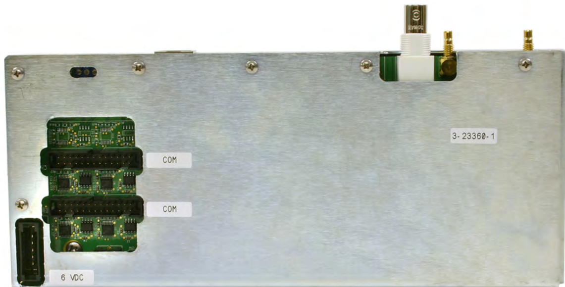
Control Board 3-23360-1 side view.
