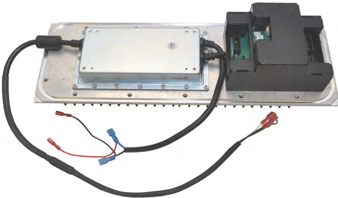
Power Supply Assembly rear view (part # 3-25381).
