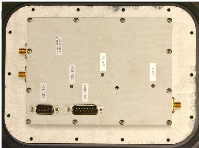
Power Amplifier 3-25406 top view
