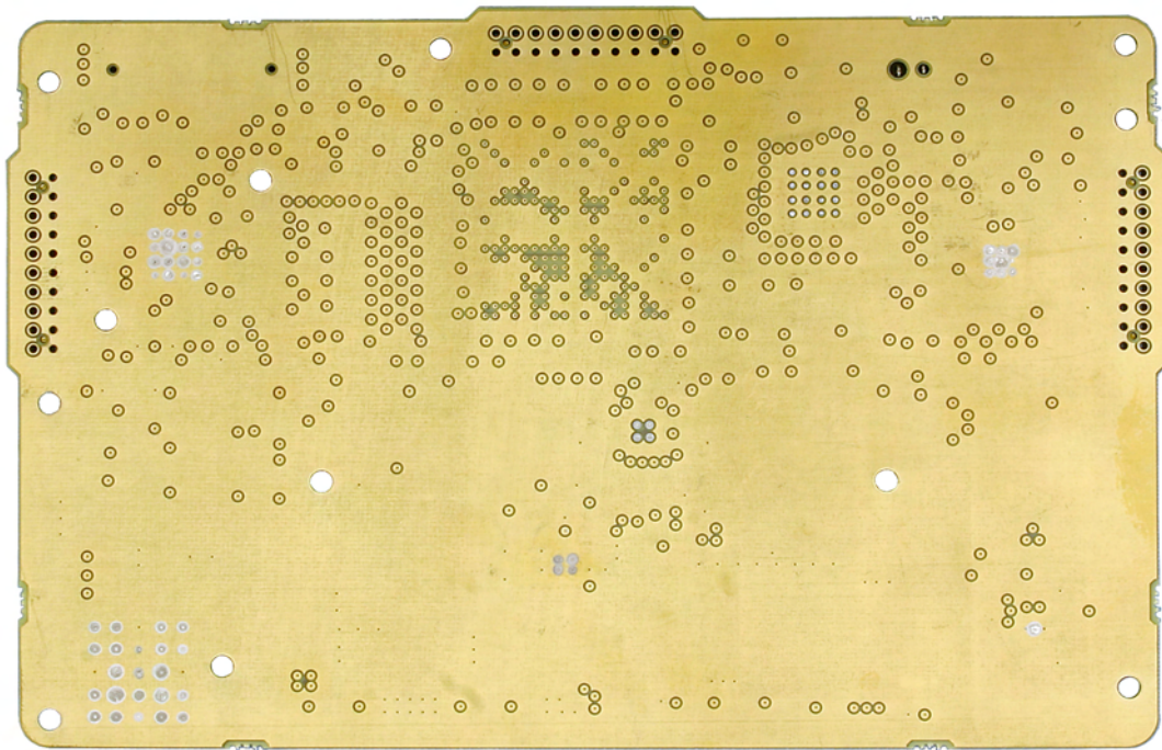
Channel Module - Digital Board 3-22310 bottom view.
