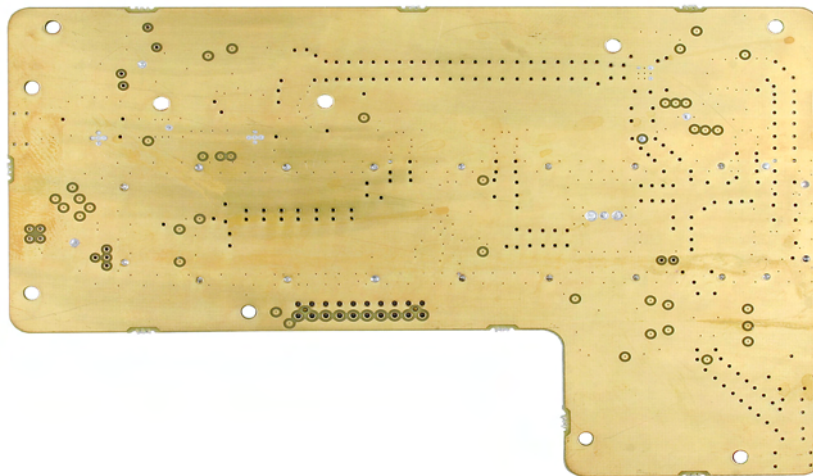
Channel Module - Down Converter Board 3-22308 bottom view.
