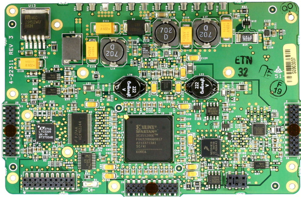
Channel Module - Digital Board 3-22310 top view.
