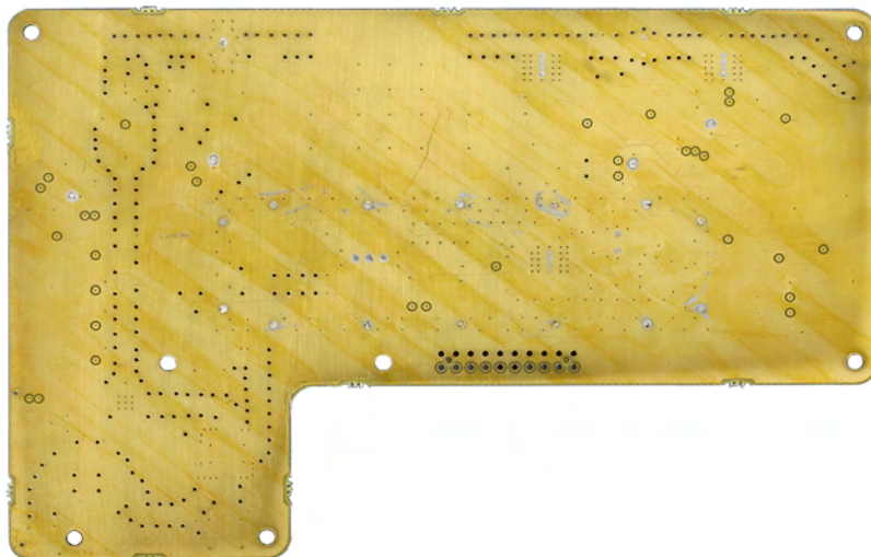
Channel Module - Up Converter Board (3-22302 or 3-22304 or 3-22306) bottom view.
