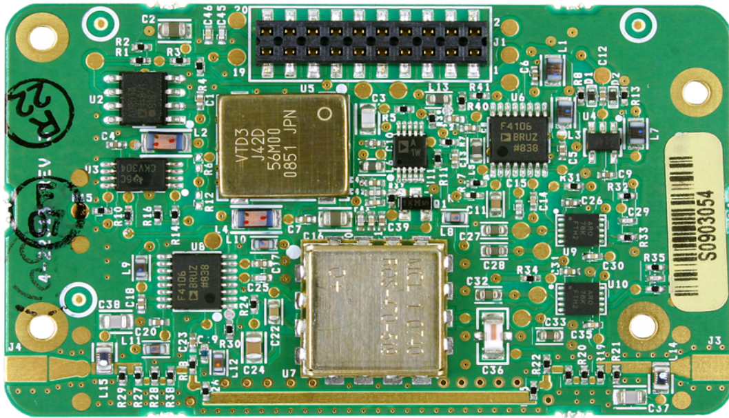
Channel Module - LO Board 3-22312 top view.
