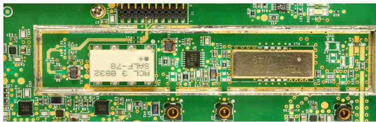
Channel Module - Down Converter Board 3-22308 under RF shield view.
