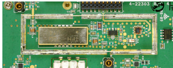
Channel Module - Up Converter Board (3-22302 or 3-22304 or 3-22306) under RF shield view.
