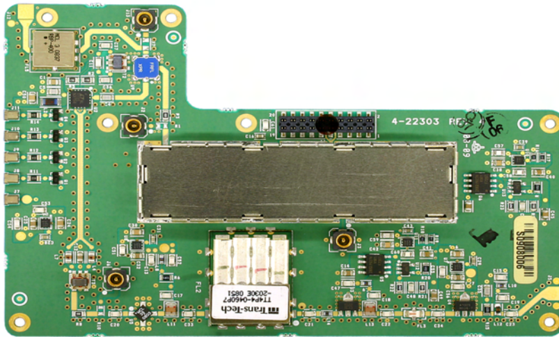
Channel Module - Up Converter Board (3-22302 or 3-22304 or 3-22306) top view.
