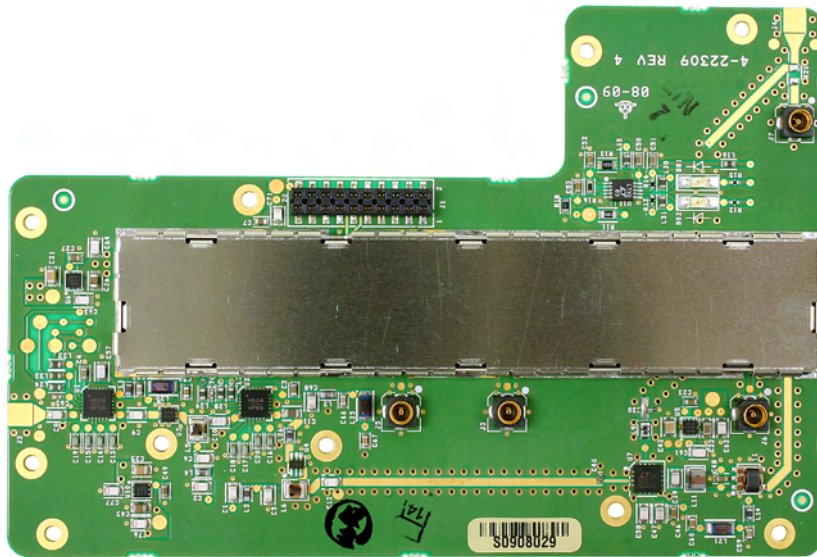
Channel Module - Down Converter Board 3-22308 top view.
