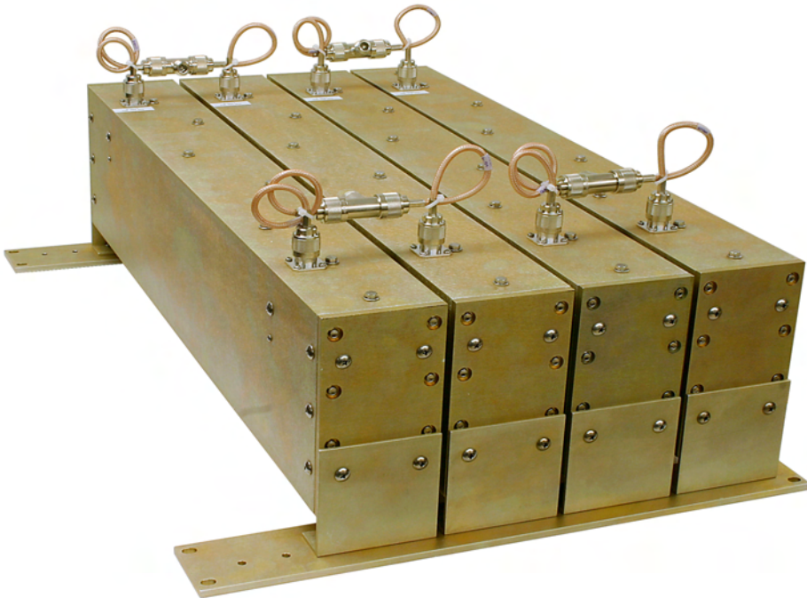
Comblin Filter Assembly 3-9774 left side view.
