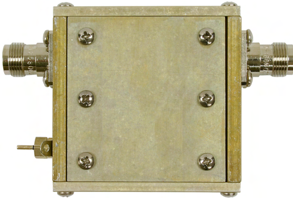
UHF Distribution Amplifier Assembly 3-22340 bottom view.
