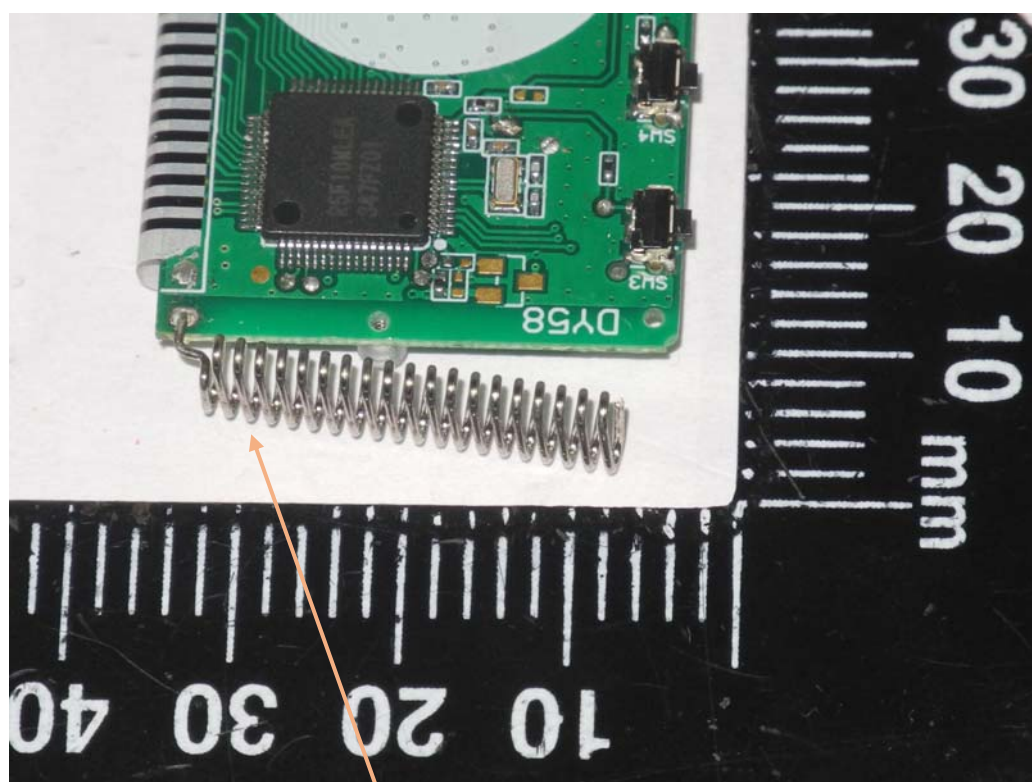
Antenna location
