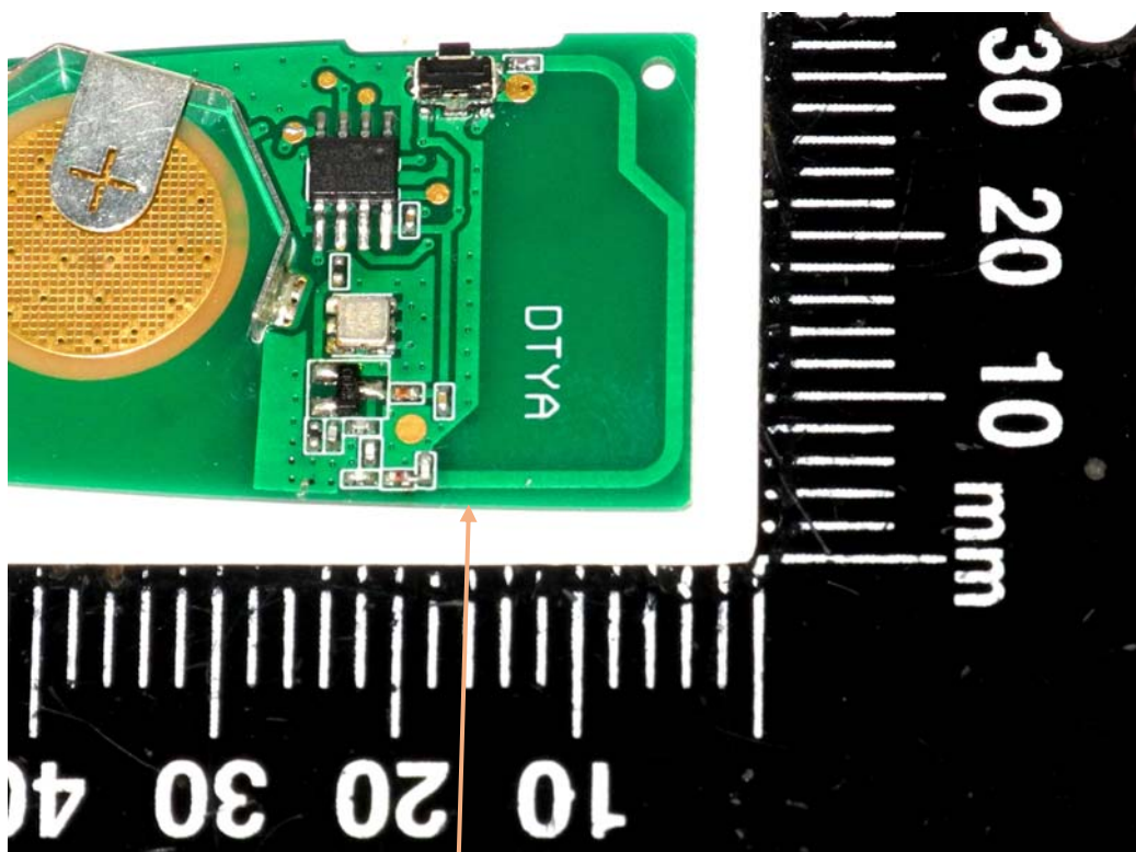
Antenna location
