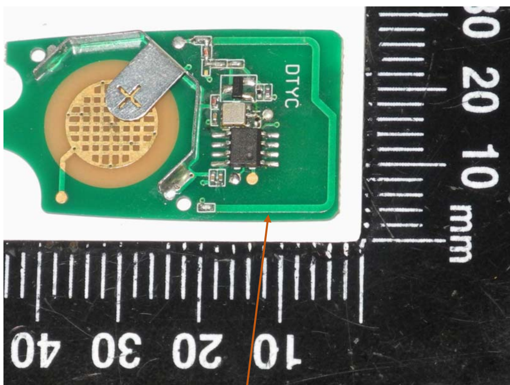
Antenna location
