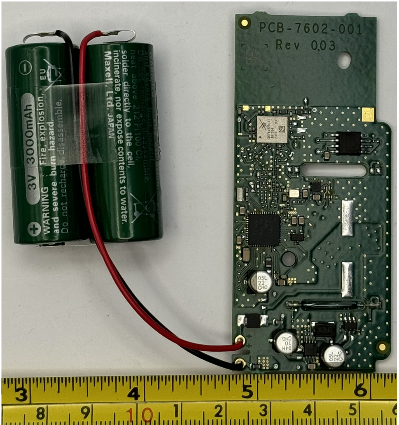
Figure 1.1: PCB Front
