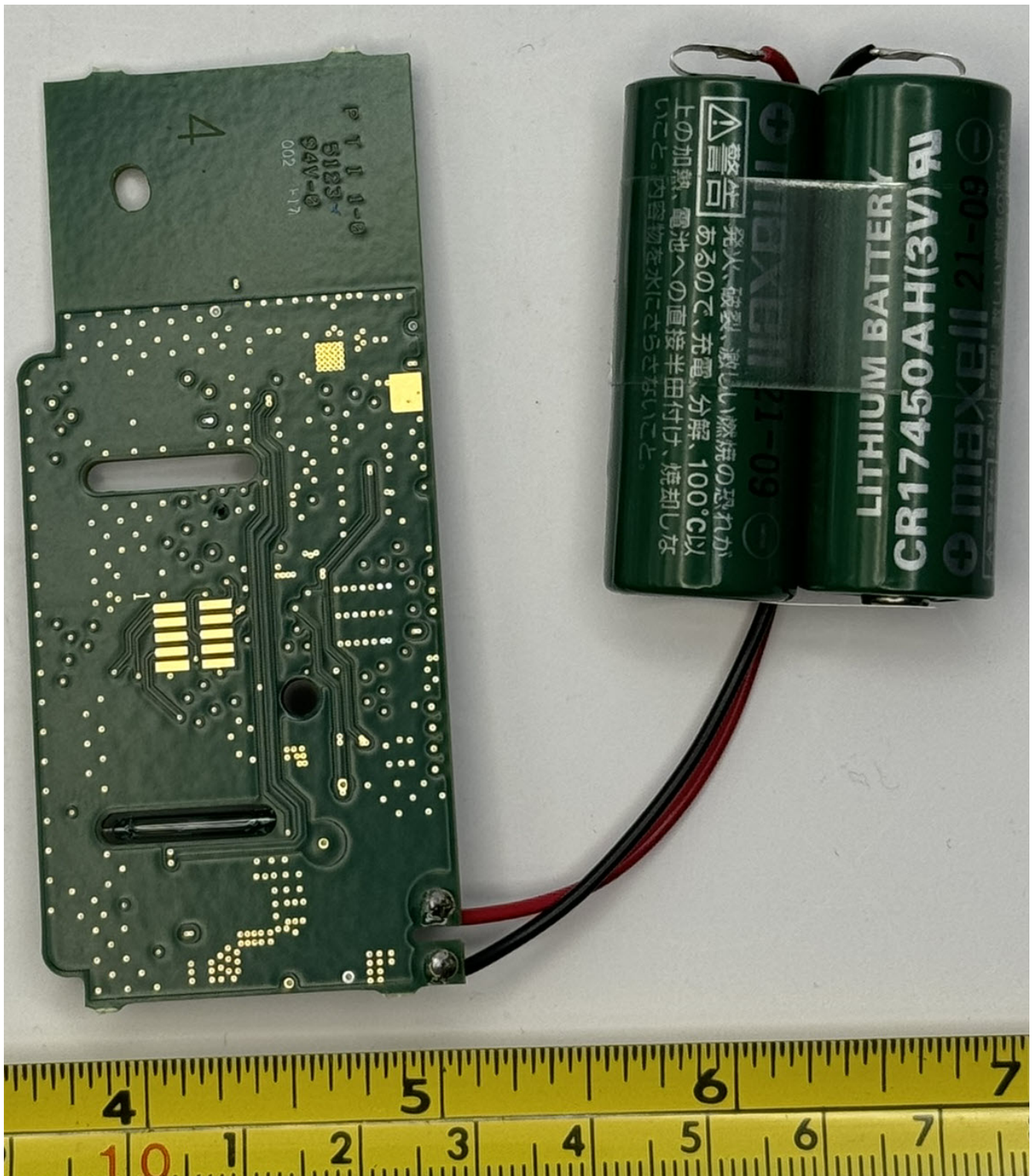
Figure 1.2: PCB Back
