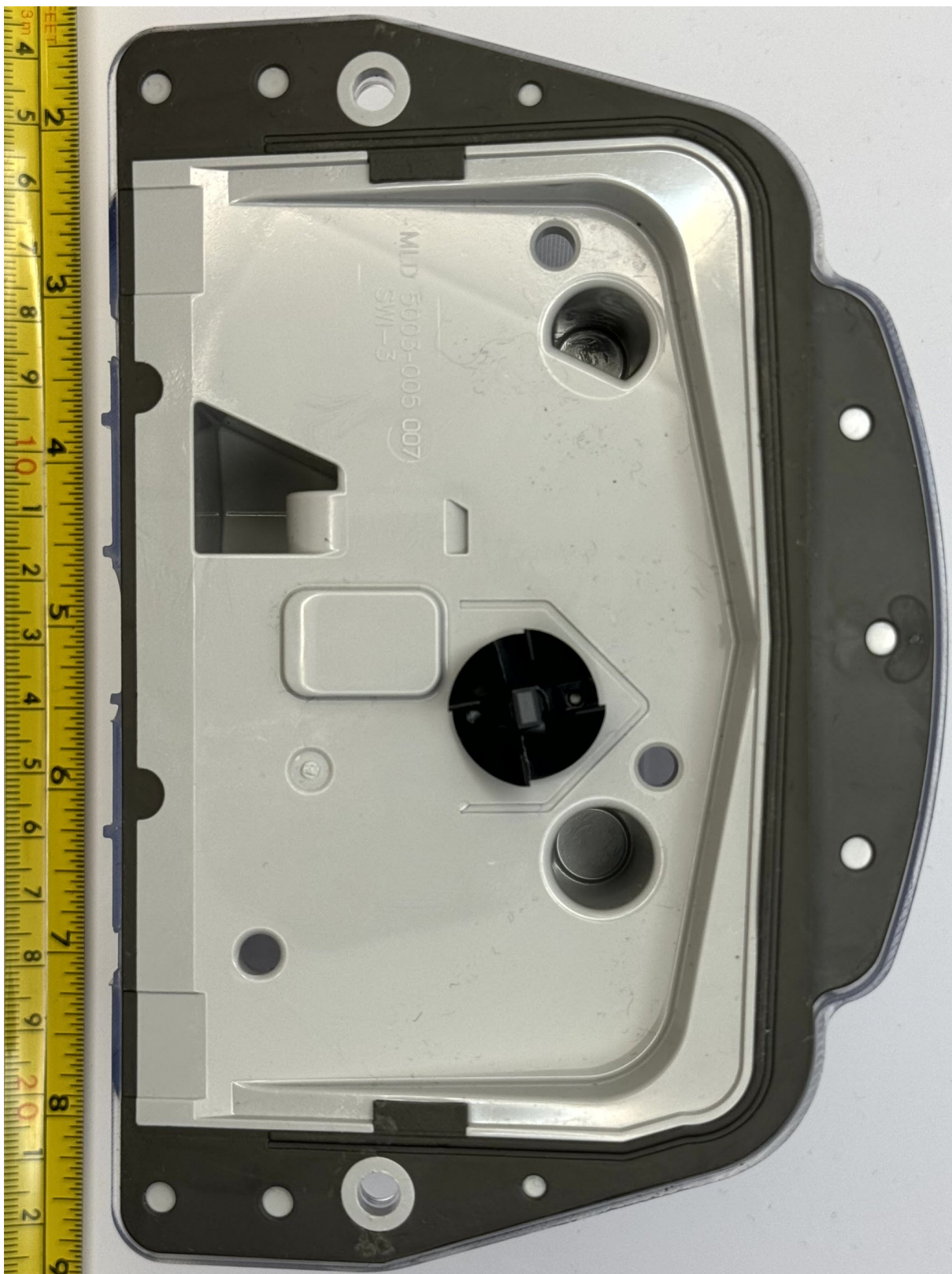
Figure 2.4: ERG-7600-005 External Back
