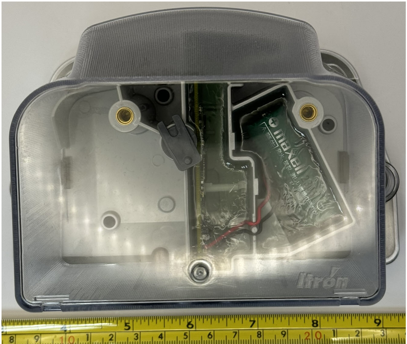
Figure 2.1: ERG-7600-005 External Front
