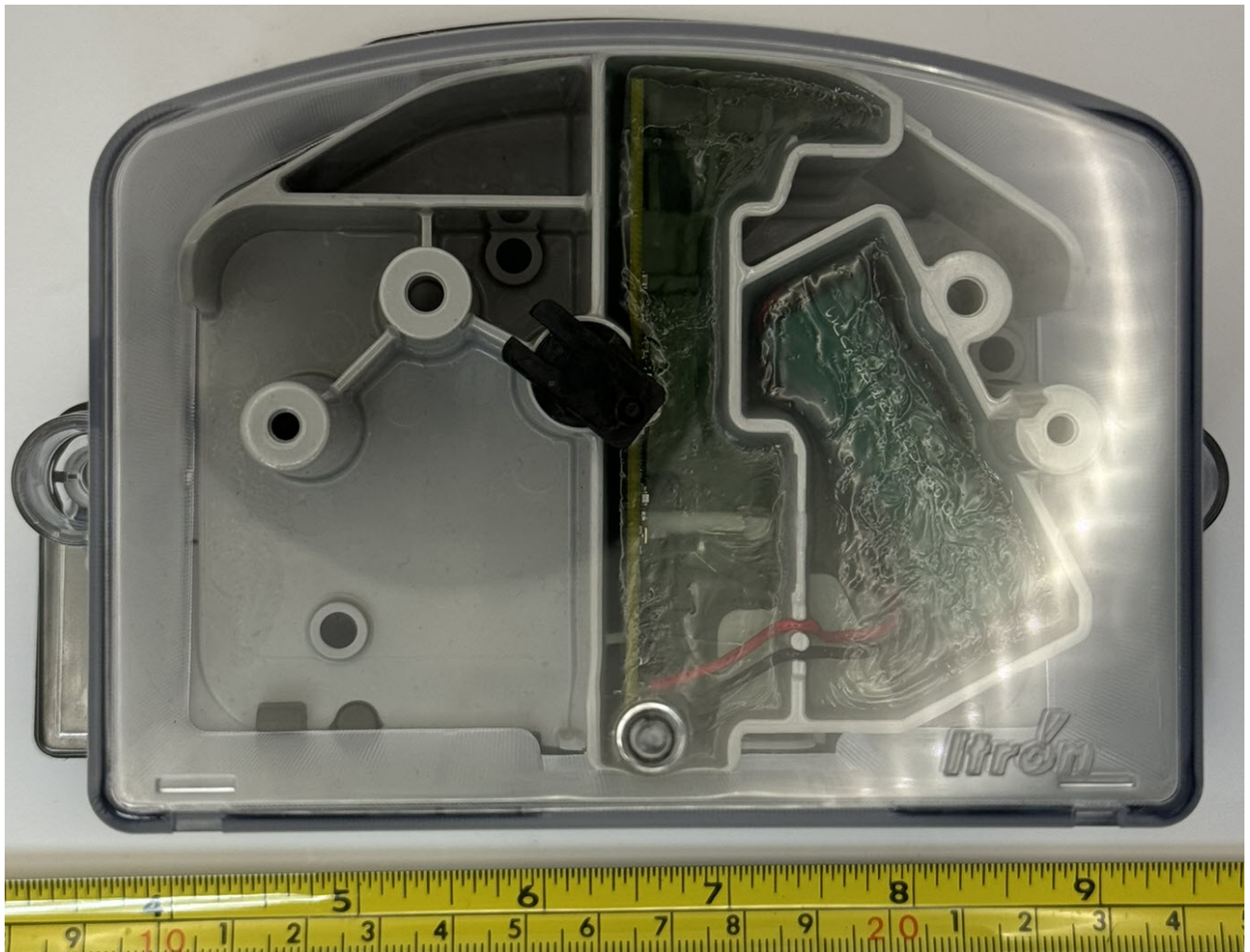
Figure 3.1: ERG-7600-006 External Front
