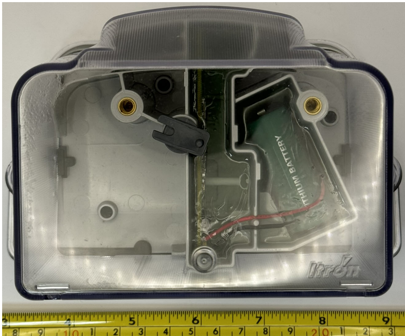
Figure 4.1: ERG-7600-010 External Front
