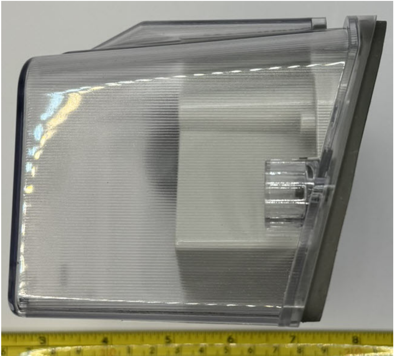
Figure 4.3: ERG-7600-010 External Right
