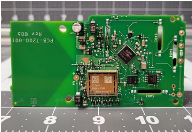
Figure 1: Component Side Overall View
