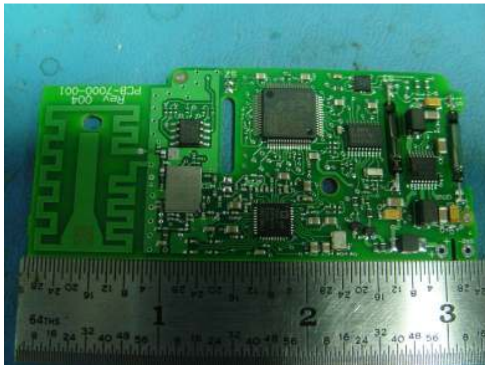
Figure 1 Top Side
